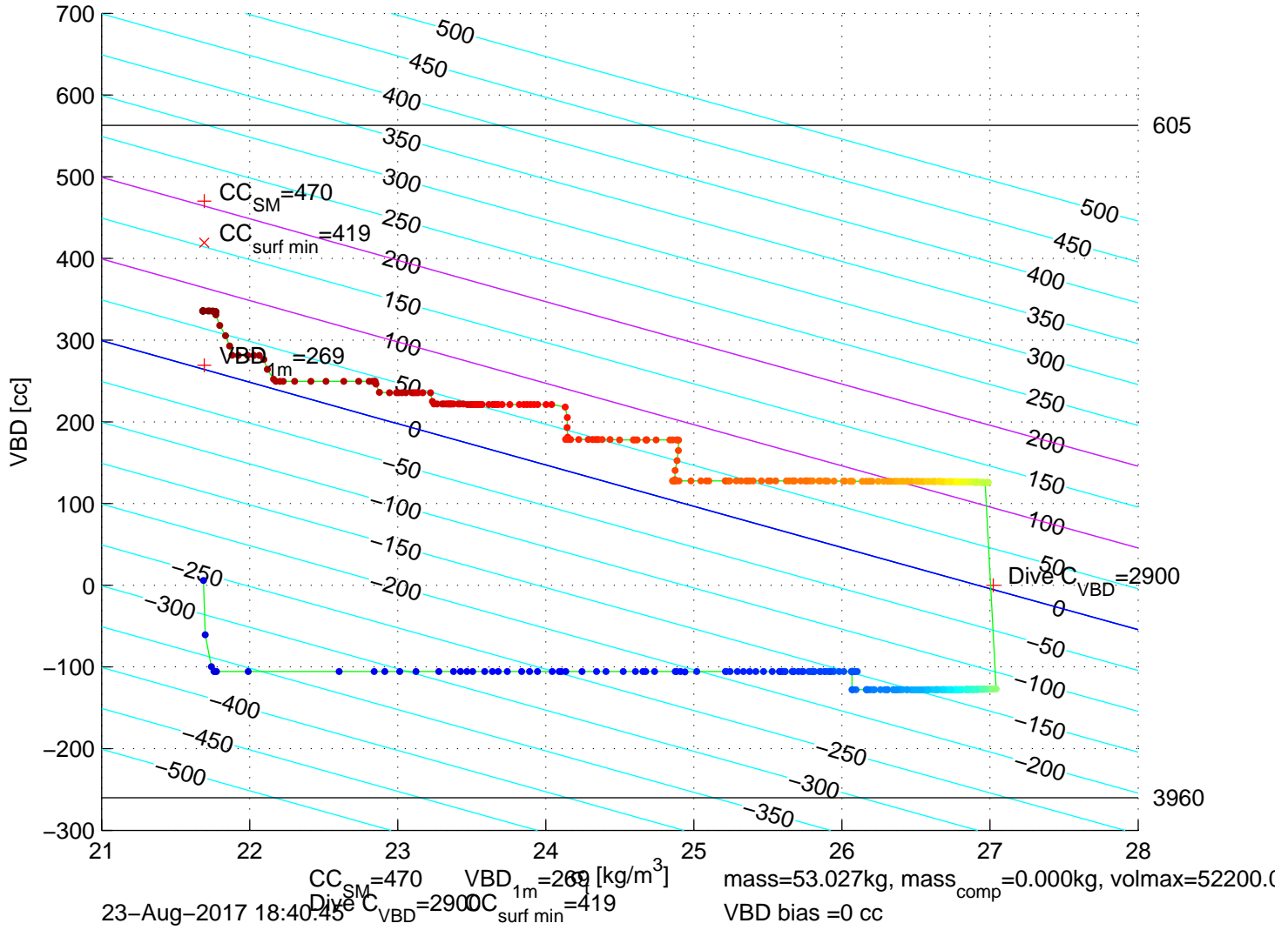
p6300310: SG630 Mission 7 Jul 2017 23-Aug-2017 20:25:20Z – buoyancy contoured
