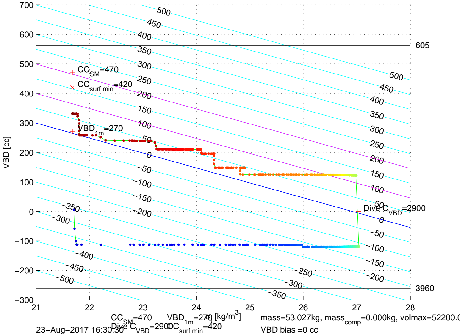
p6300309: SG630 Mission 7 Jul 2017 23-Aug-2017 18:23:59Z – buoyancy contoured
