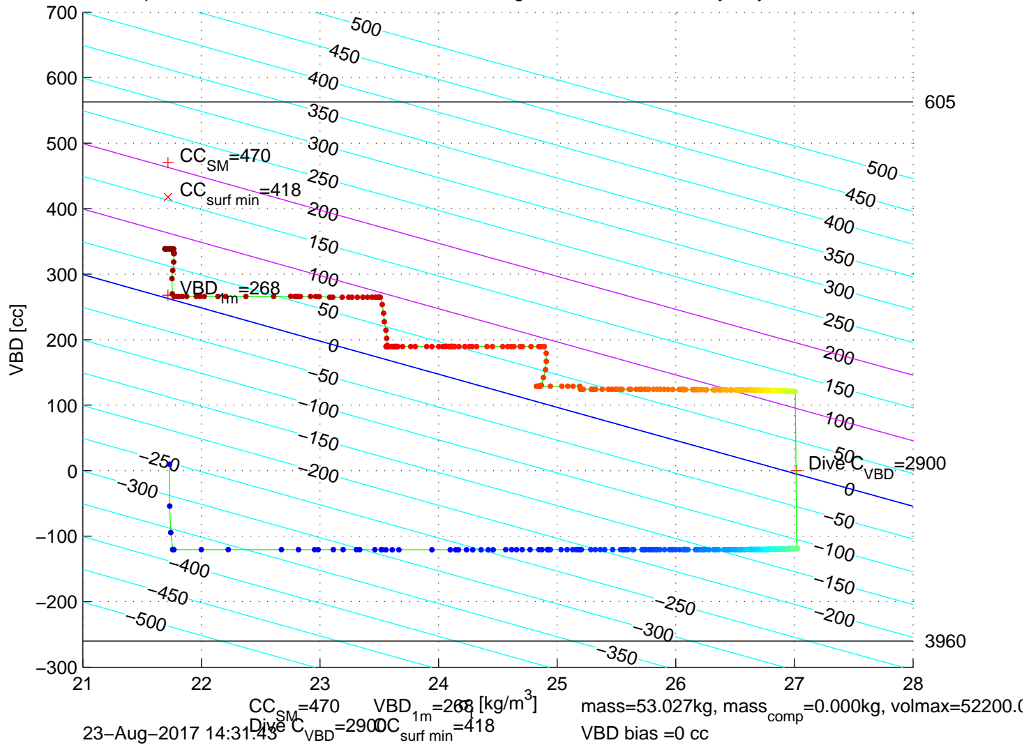
p6300308: SG630 Mission 7 Jul 2017 23-Aug-2017 16:20:39Z – buoyancy contoured
