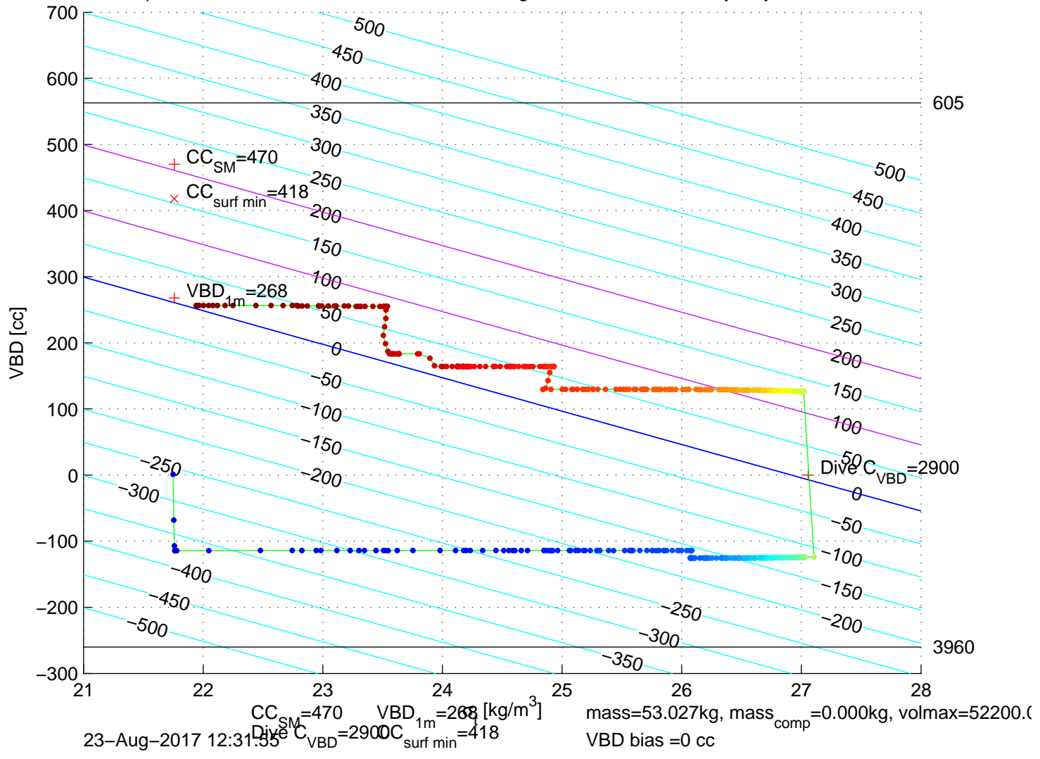
p6300307: SG630 Mission 7 Jul 2017 23-Aug-2017 14:11:35Z – buoyancy contoured
