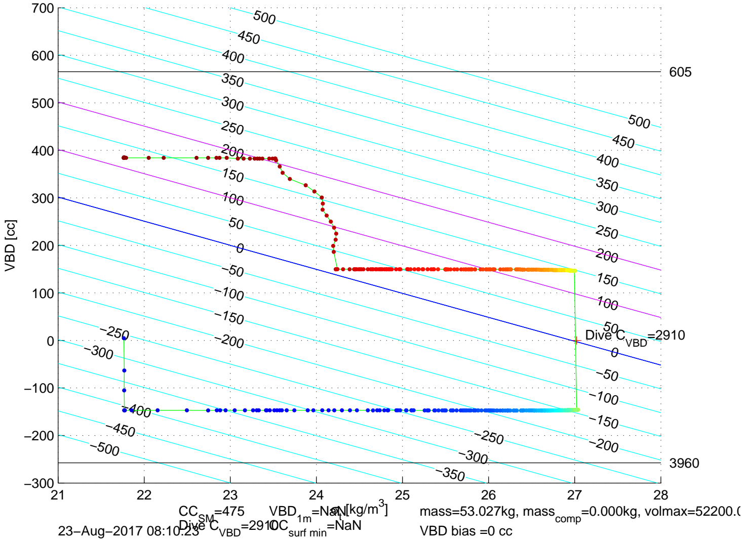
p6300305: SG630 Mission 7 Jul 2017 23-Aug-2017 10:08:24Z – buoyancy contoured
