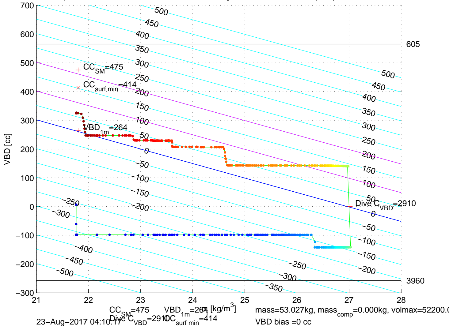
p6300303: SG630 Mission 7 Jul 2017 23-Aug-2017 06:03:17Z – buoyancy contoured
