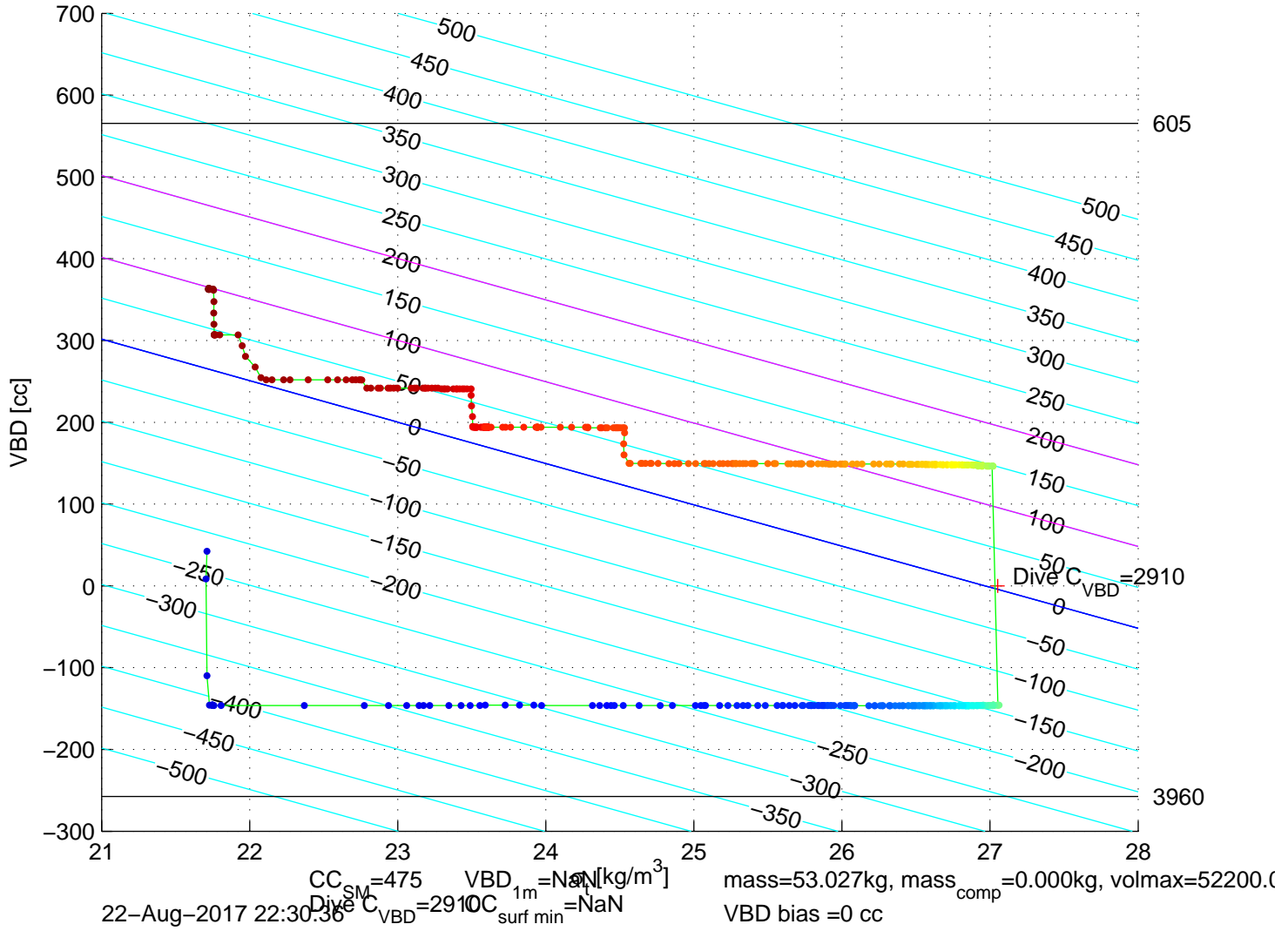
p6300300: SG630 Mission 7 Jul 2017 22-Aug-2017 23:29:41Z – buoyancy contoured
