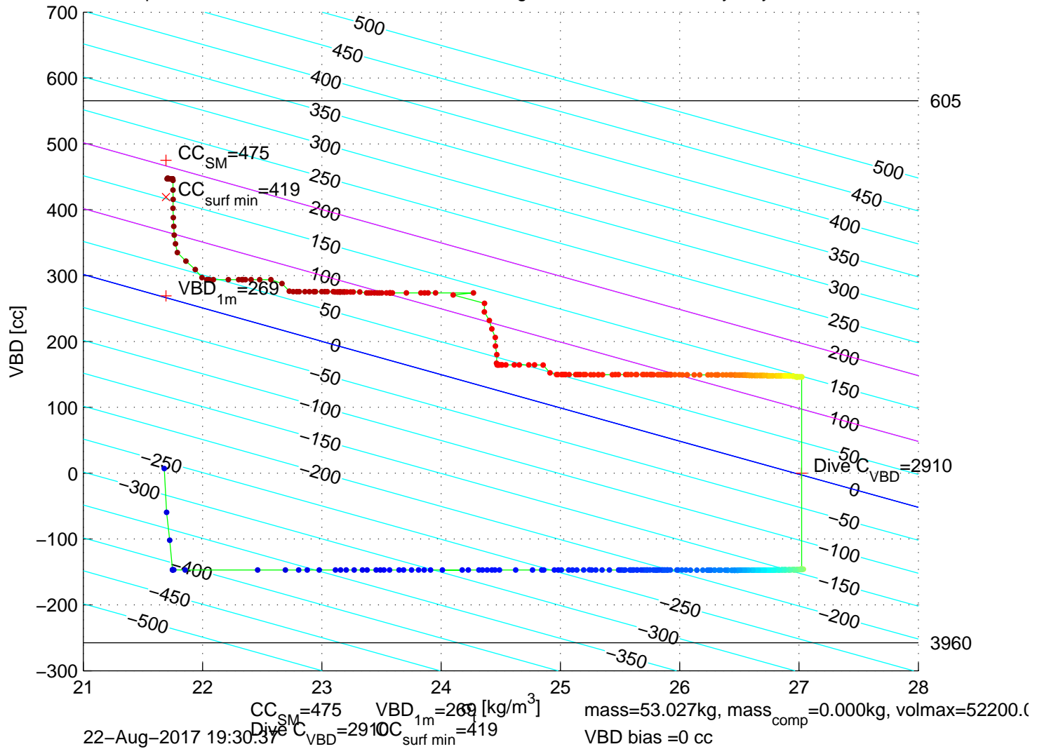
p6300299: SG630 Mission 7 Jul 2017 22-Aug-2017 21:26:47Z – buoyancy contoured
