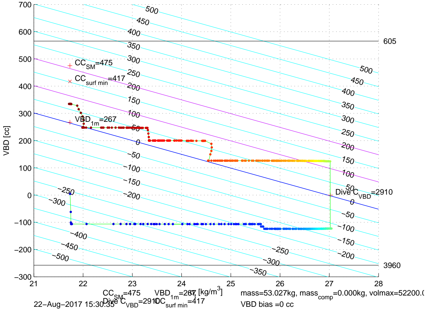
p6300296: SG630 Mission 7 Jul 2017 22-Aug-2017 14:54:28Z – buoyancy contoured
