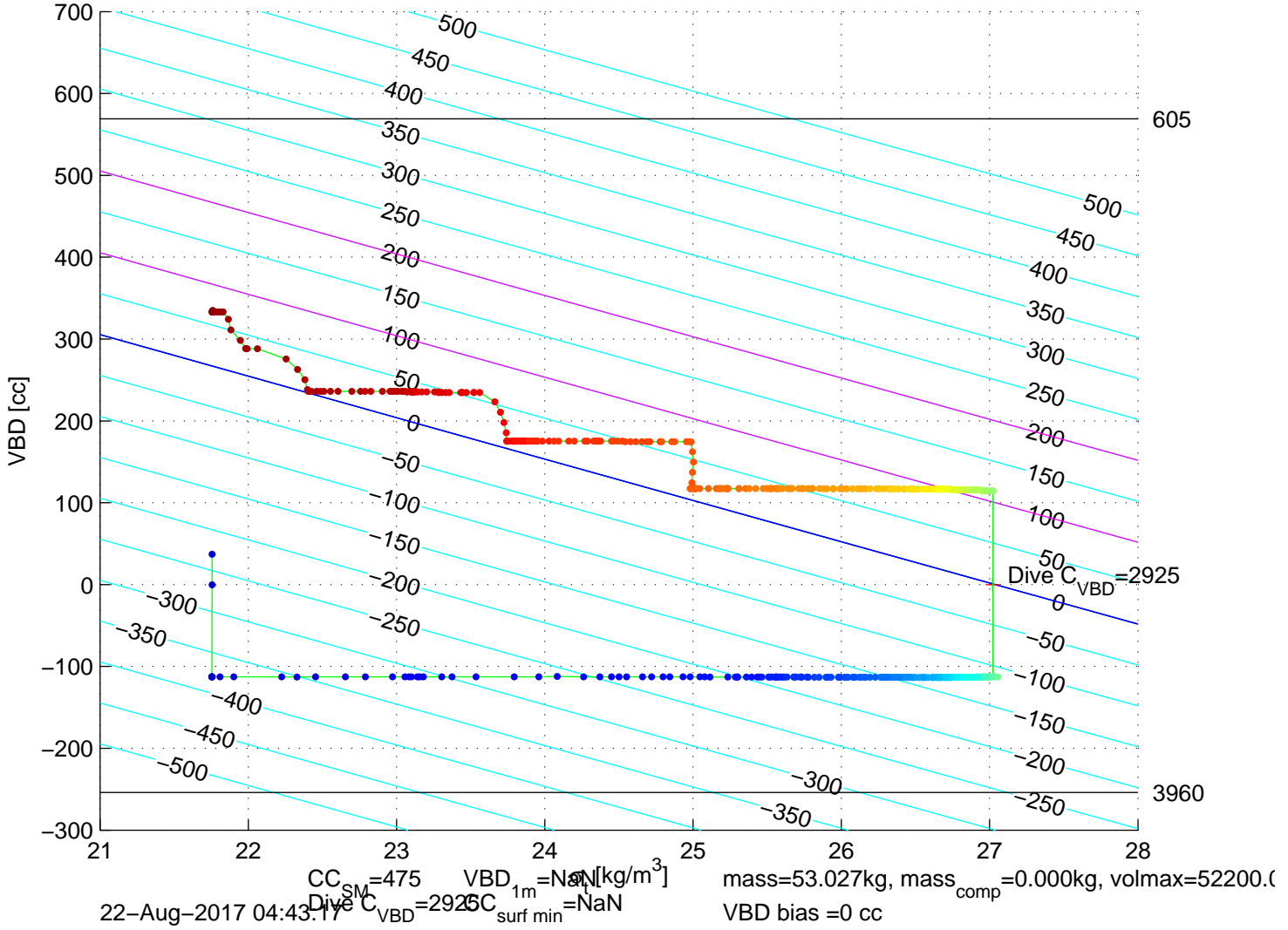
p6300292: SG630 Mission 7 Jul 2017 22-Aug-2017 06:24:08Z - buoyancy contoured
