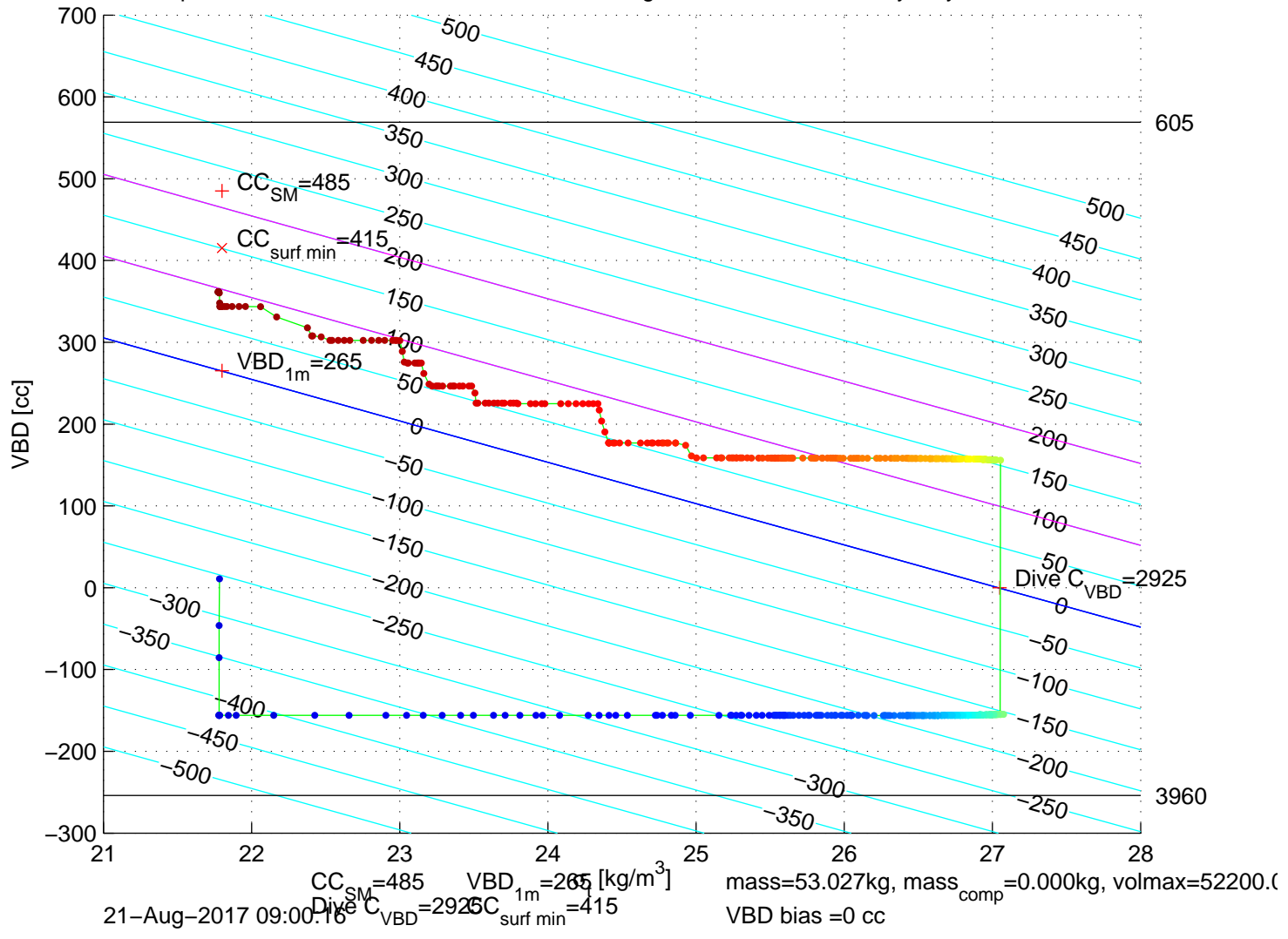
p6300283: SG630 Mission 7 Jul 2017 21-Aug-2017 10:54:35Z – buoyancy contoured
