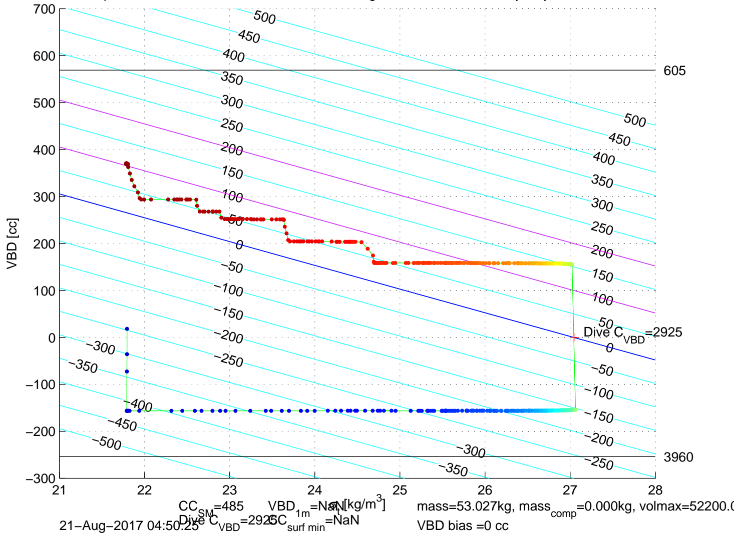
p6300281: SG630 Mission 7 Jul 2017 21-Aug-2017 06:39:54Z – buoyancy contoured
