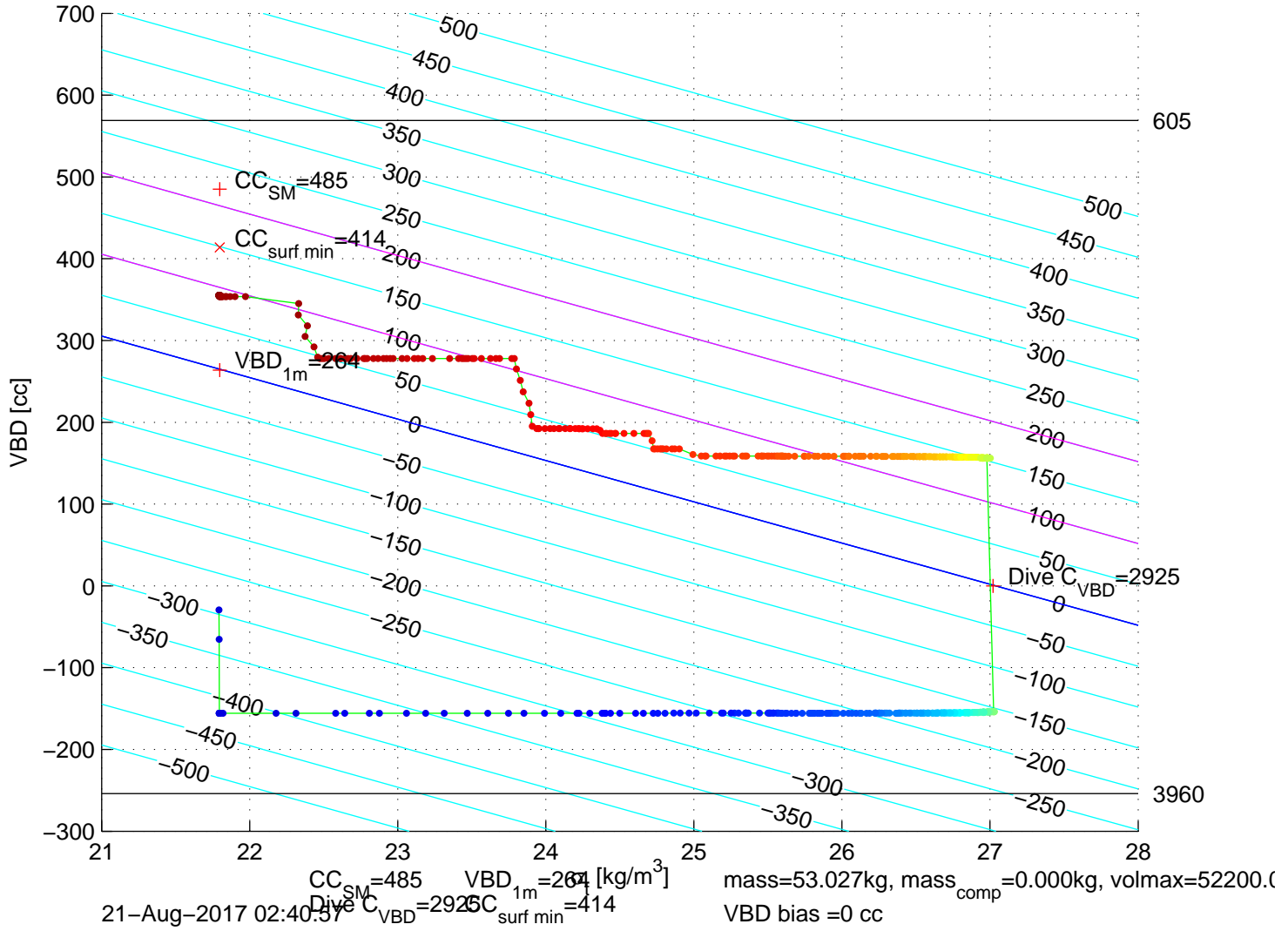
p6300280: SG630 Mission 7 Jul 2017 21-Aug-2017 04:19:45Z – buoyancy contoured
