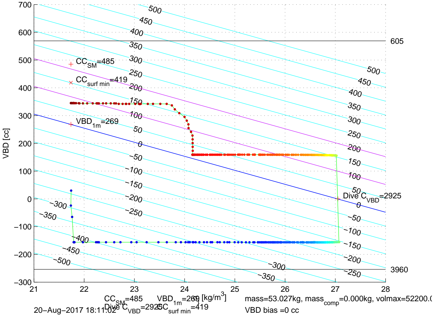
p6300276: SG630 Mission 7 Jul 2017 20-Aug-2017 20:03:40Z – buoyancy contoured
