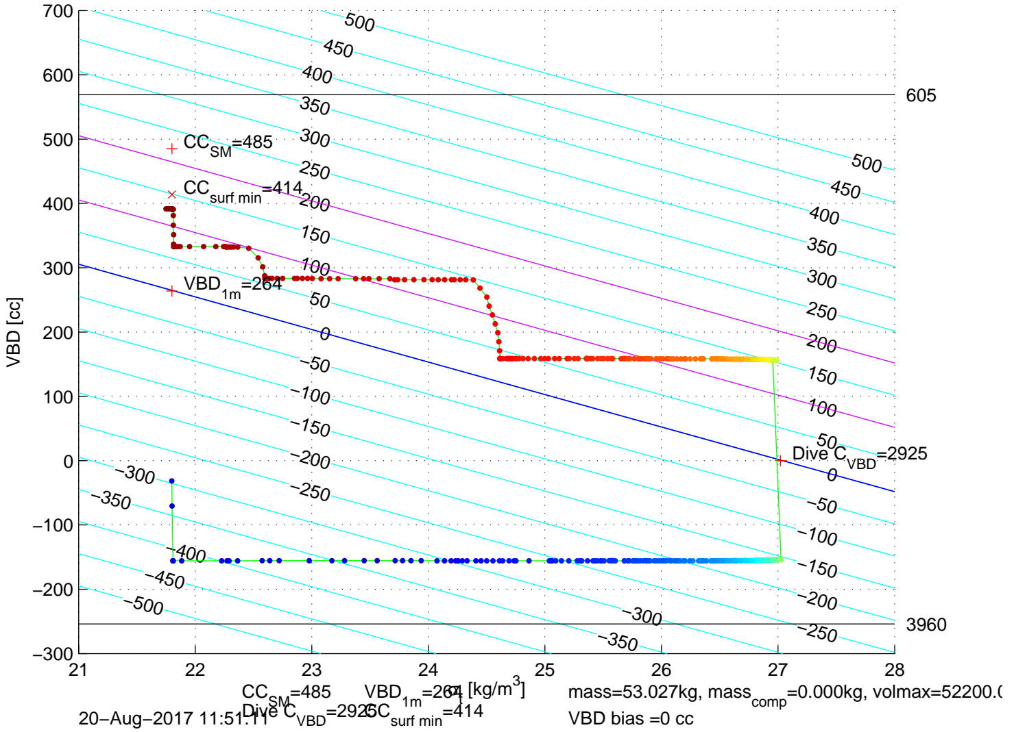
p6300273: SG630 Mission 7 Jul 2017 20-Aug-2017 13:34:46Z – buoyancy contoured
