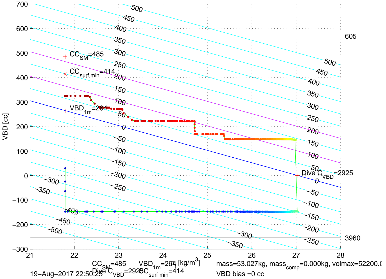
p6300267: SG630 Mission 7 Jul 2017 20-Aug-2017 00:24:42Z – buoyancy contoured
