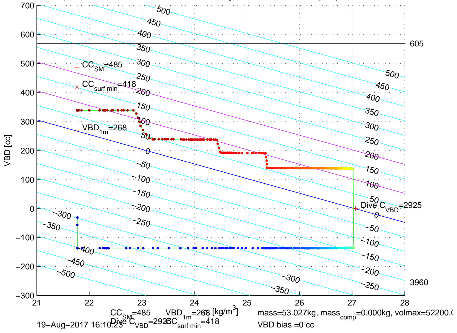
p6300264: SG630 Mission 7 Jul 2017 19-Aug-2017 17:57:30Z - buoyancy contoured
