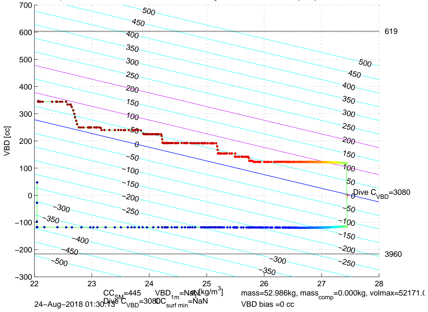
p6300260: SG630 Mission 8 Jul 2018 24-Aug-2018 01:25:21Z – buoyancy contoured
