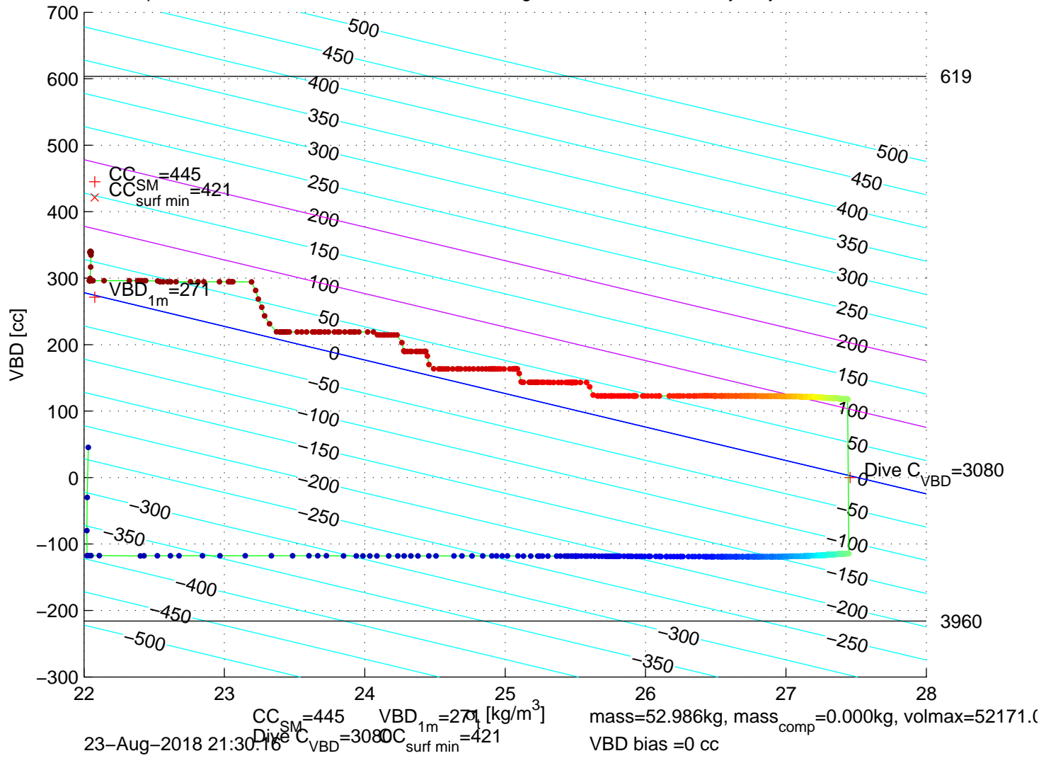
p6300259: SG630 Mission 8 Jul 2018 23-Aug-2018 21:29:25Z – buoyancy contoured
