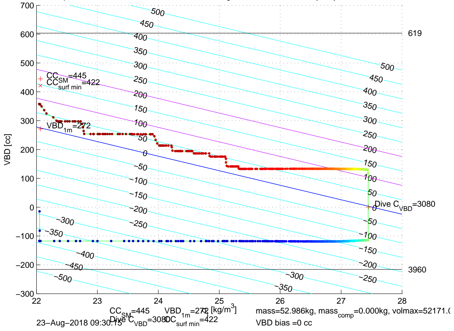
p6300256: SG630 Mission 8 Jul 2018 23-Aug-2018 09:37:46Z – buoyancy contoured
