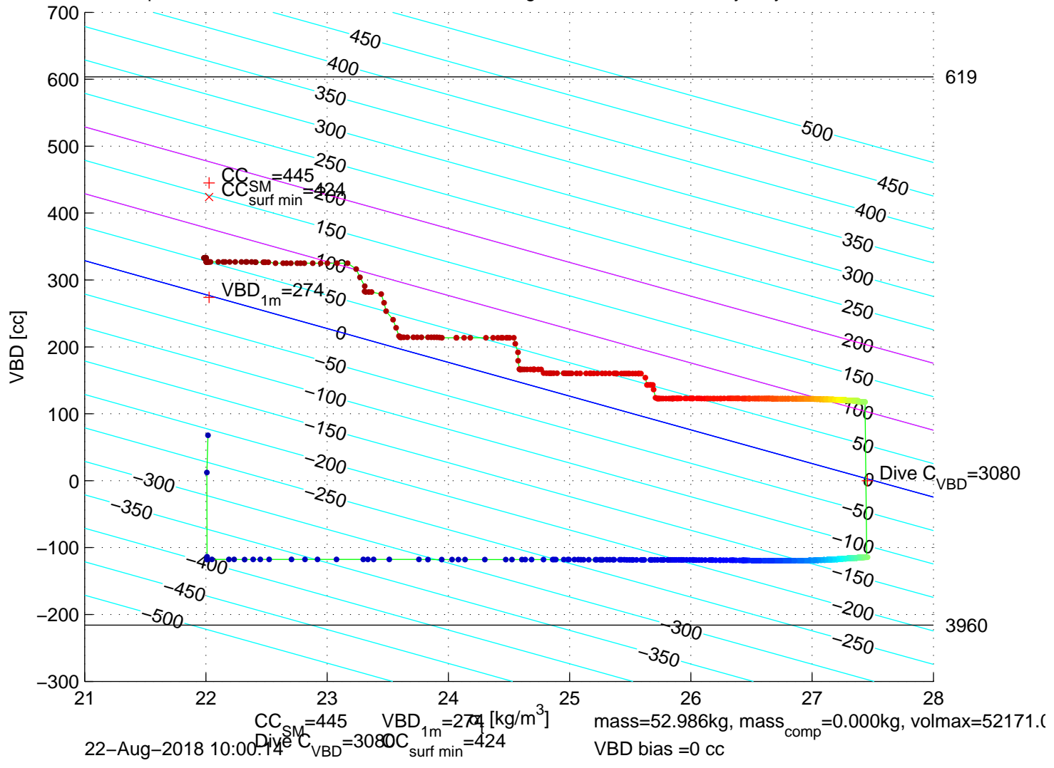
p6300250: SG630 Mission 8 Jul 2018 22-Aug-2018 09:53:02Z – buoyancy contoured
