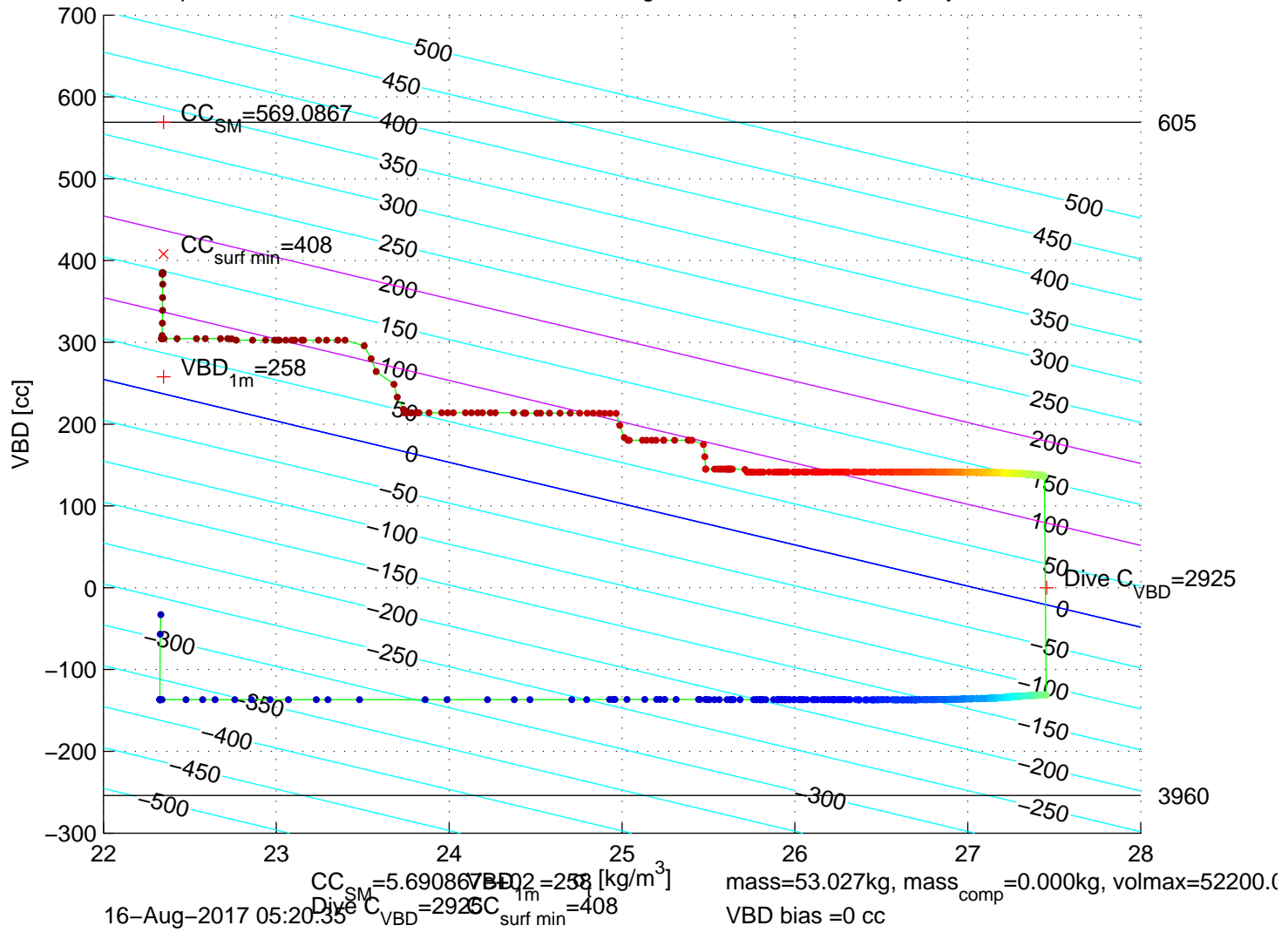
p6300239: SG630 Mission 7 Jul 16–Aug–2017 05:21:28Z – buoyancy contoured
