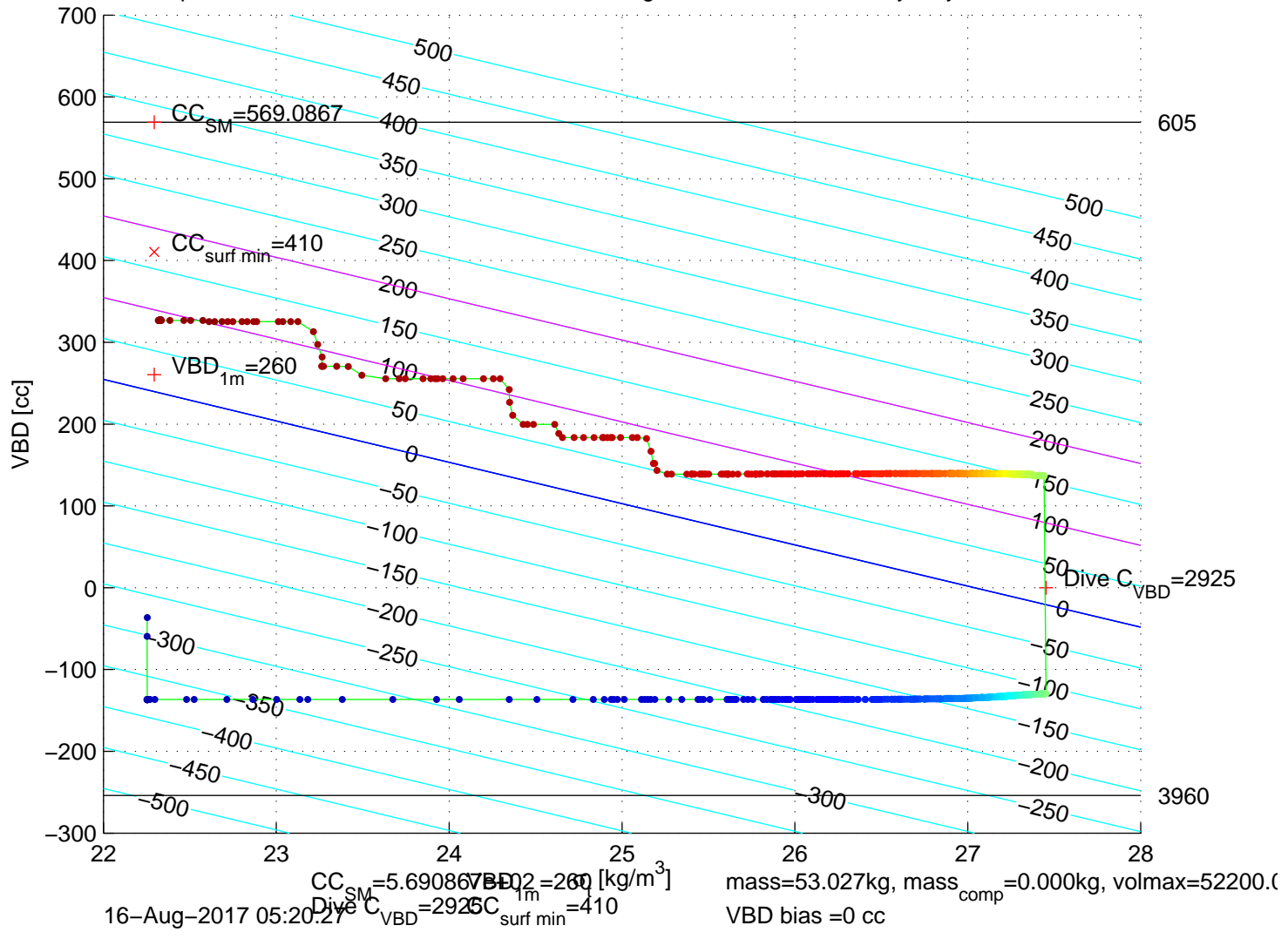
p6300238: SG630 Mission 7 Jul 2017 16–Aug–2017 01:32:07Z – buoyancy contoured
