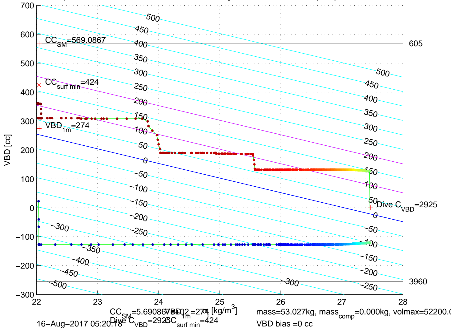
p6300235: SG630 Mission 7 Jul 2017 15–Aug–2017 13:43:39Z – buoyancy contoured
