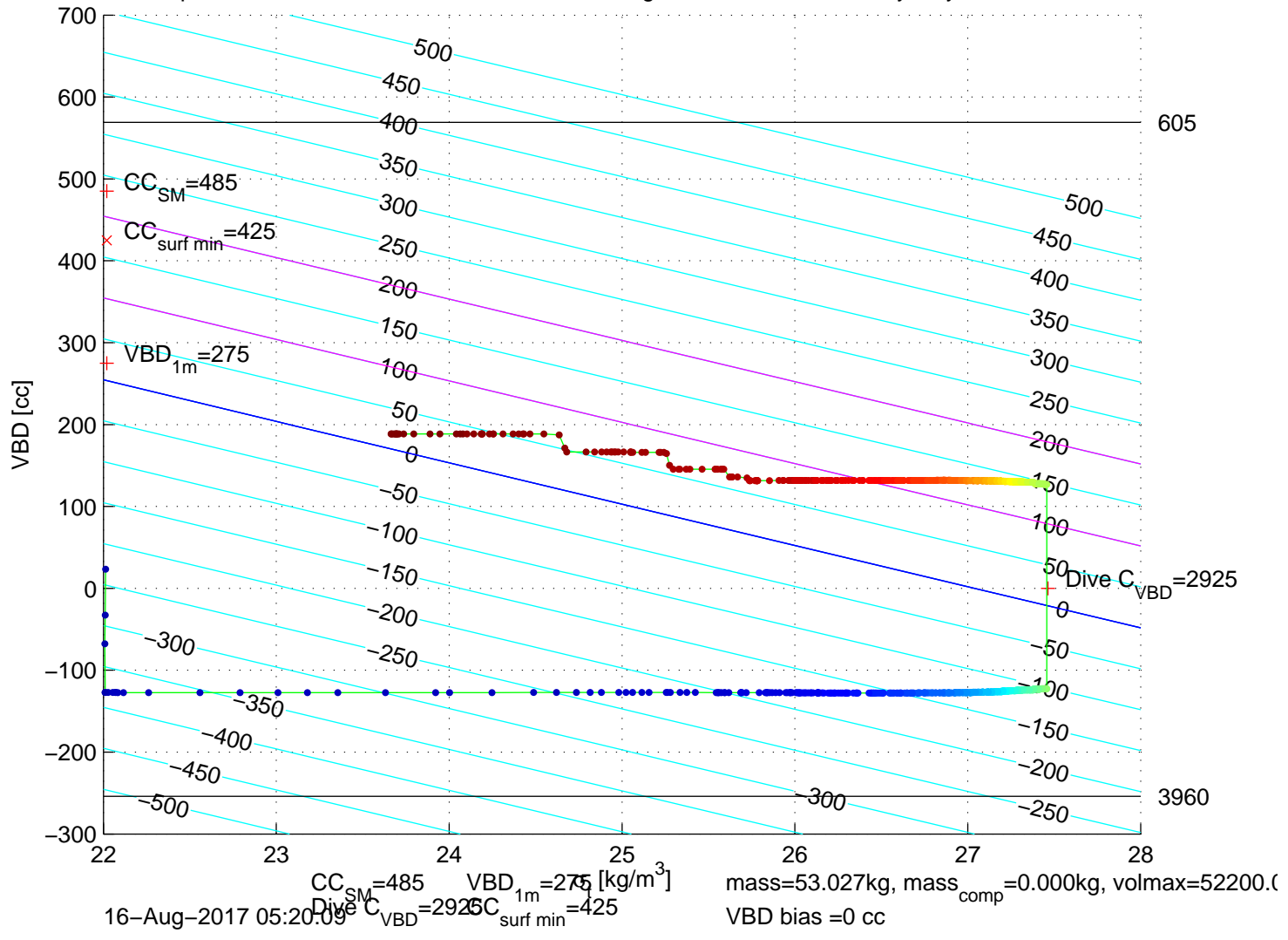
p6300234: SG630 Mission 7 Jul 2017 15–Aug–2017 09:47:45Z – buoyancy contoured
