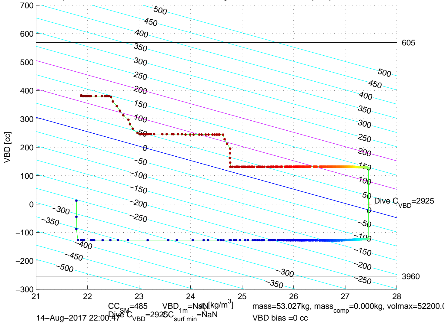
p6300231: SG630 Mission 7 Jul 2017 14-Aug-2017 21:57:44Z – buoyancy contoured
