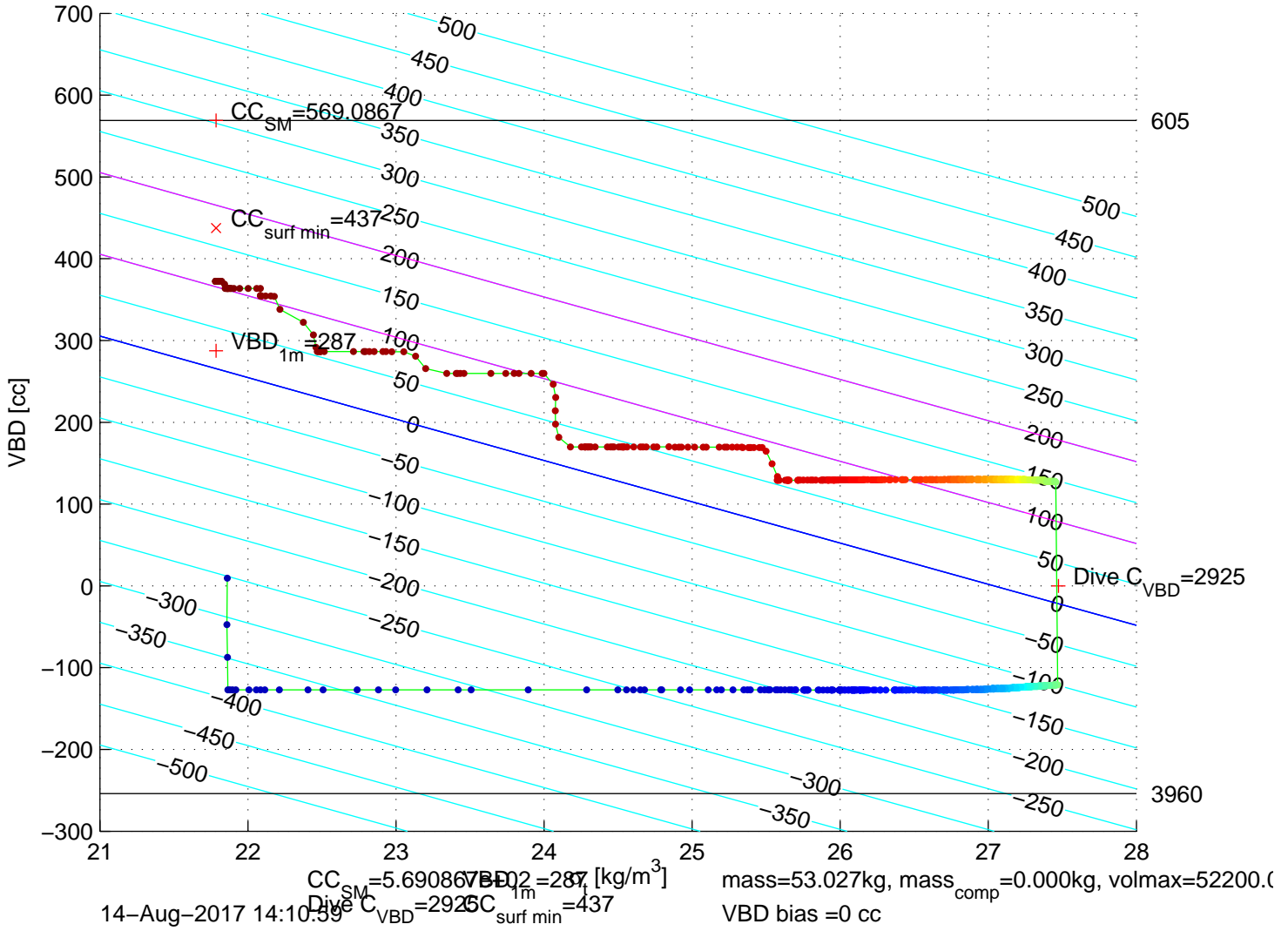
p6300229: SG630 Mission 7 Jul 2017 14-Aug-2017 14:12:21Z – buoyancy contoured
