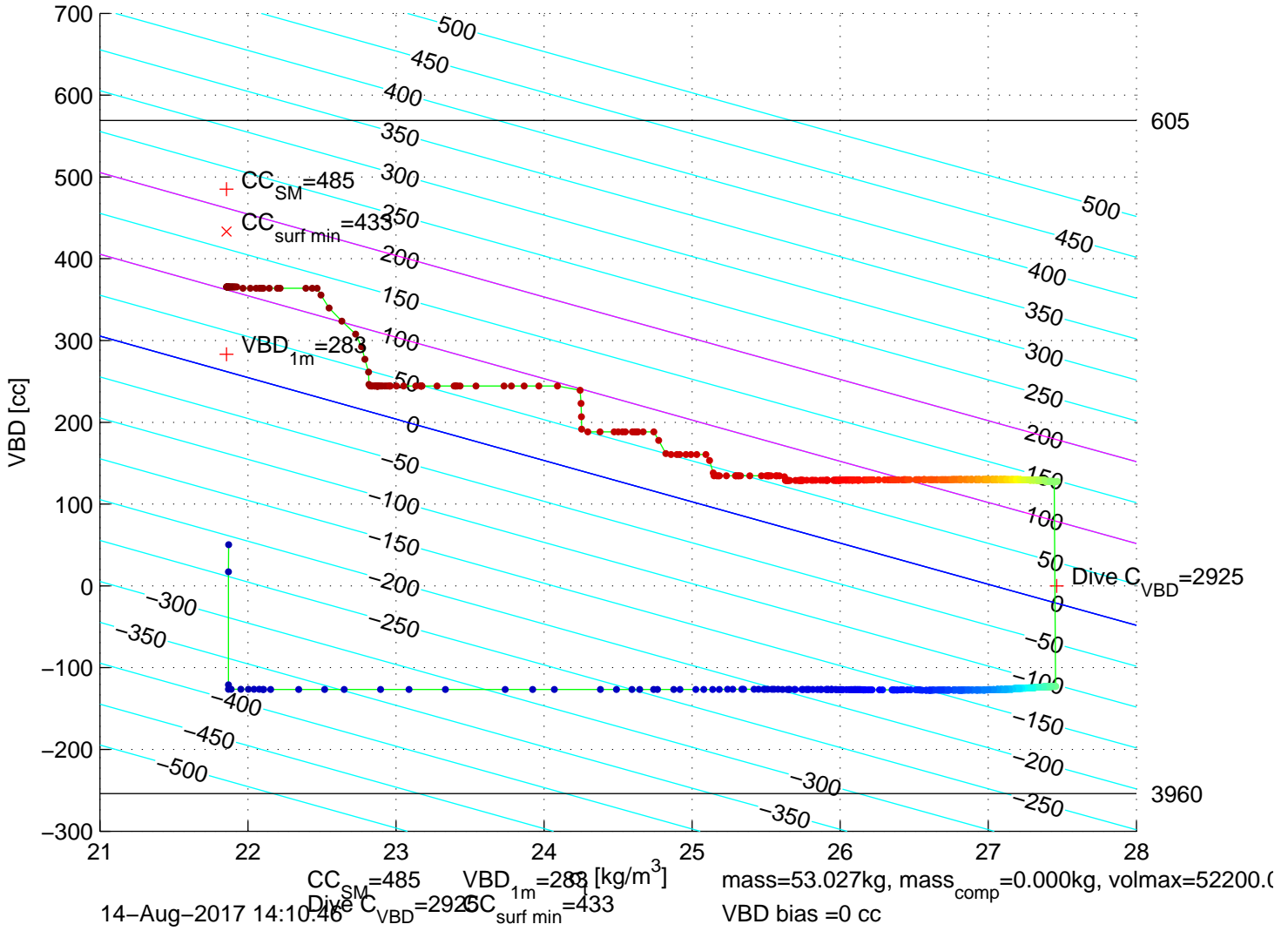
p6300228: SG630 Mission 7 Jul 2017 14-Aug-2017 10:13:40Z – buoyancy contoured
