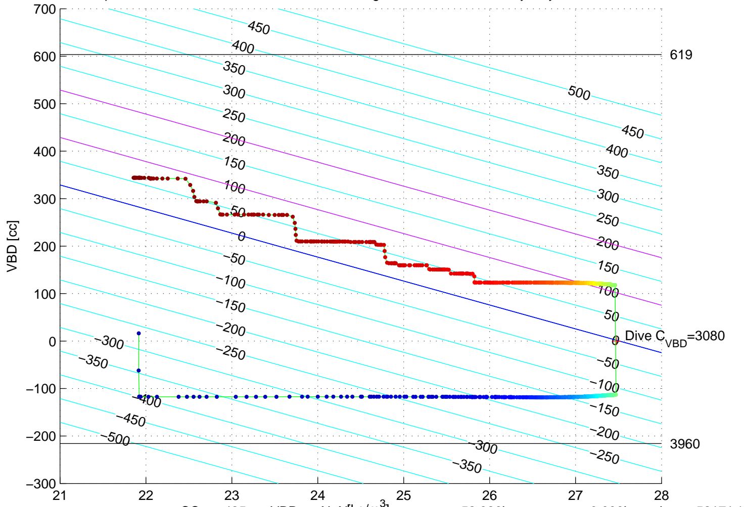
p6300227: SG630 Mission 8 Jul 2018 18-Aug-2018 14:13:00Z - buoyancy contoured
