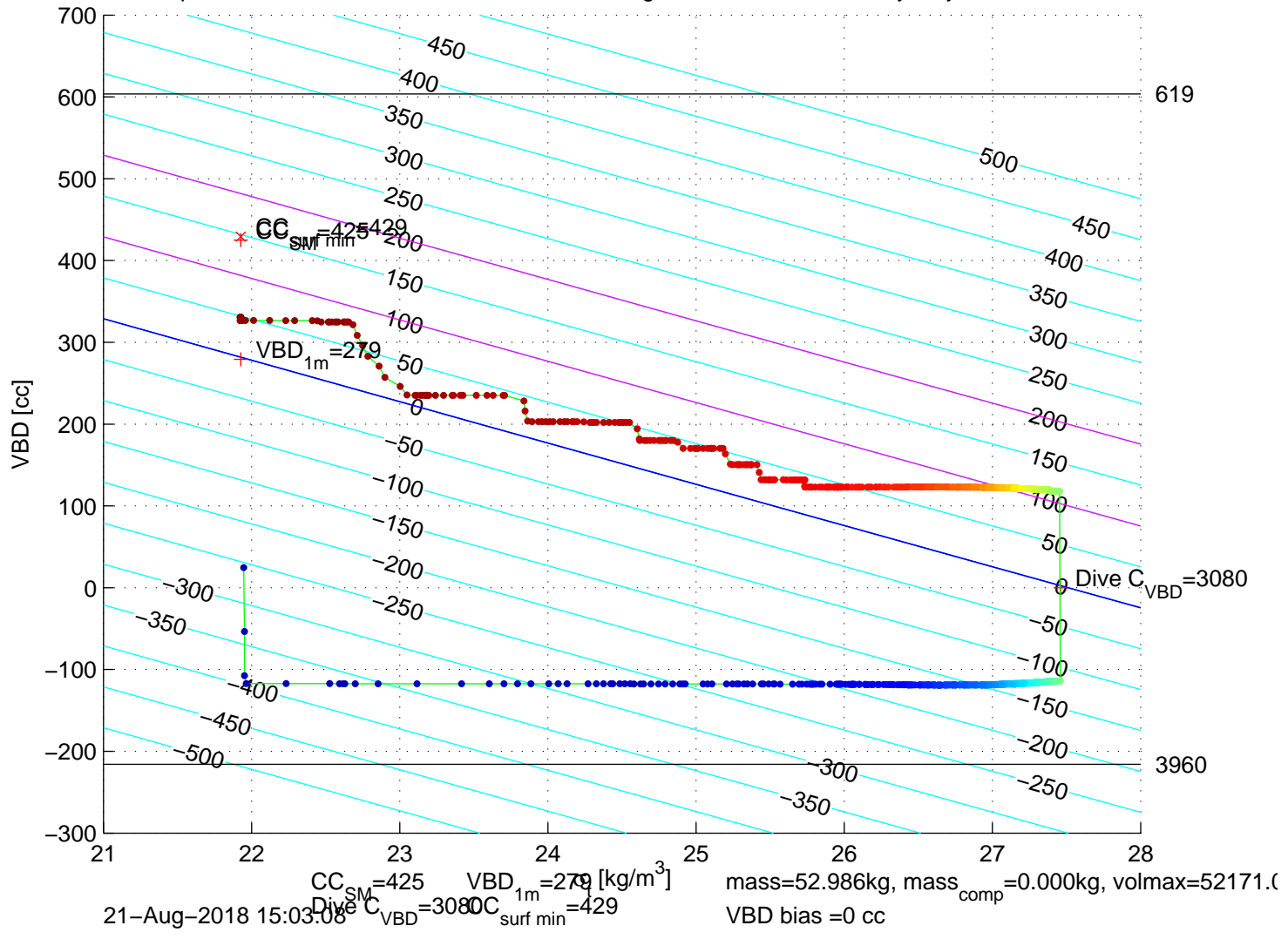
p6300225: SG630 Mission 8 Jul 2018 18-Aug-2018 06:09:48Z – buoyancy contoured
