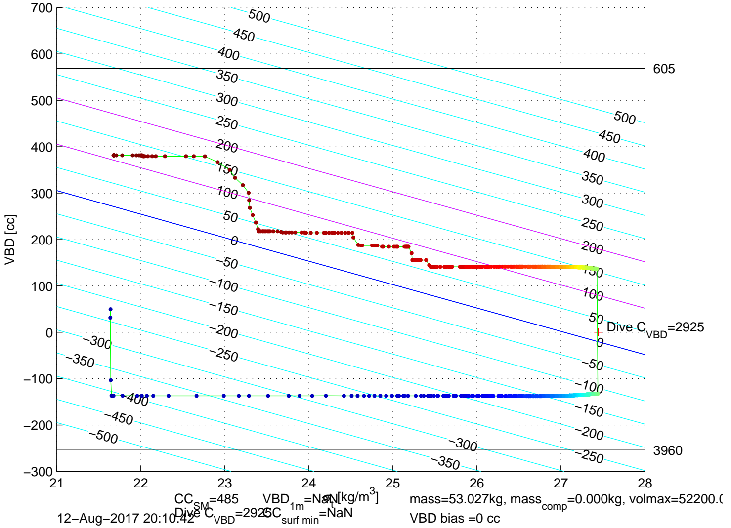
p6300218: SG630 Mission 7 Jul 2017 12-Aug-2017 20:22:53Z – buoyancy contoured
