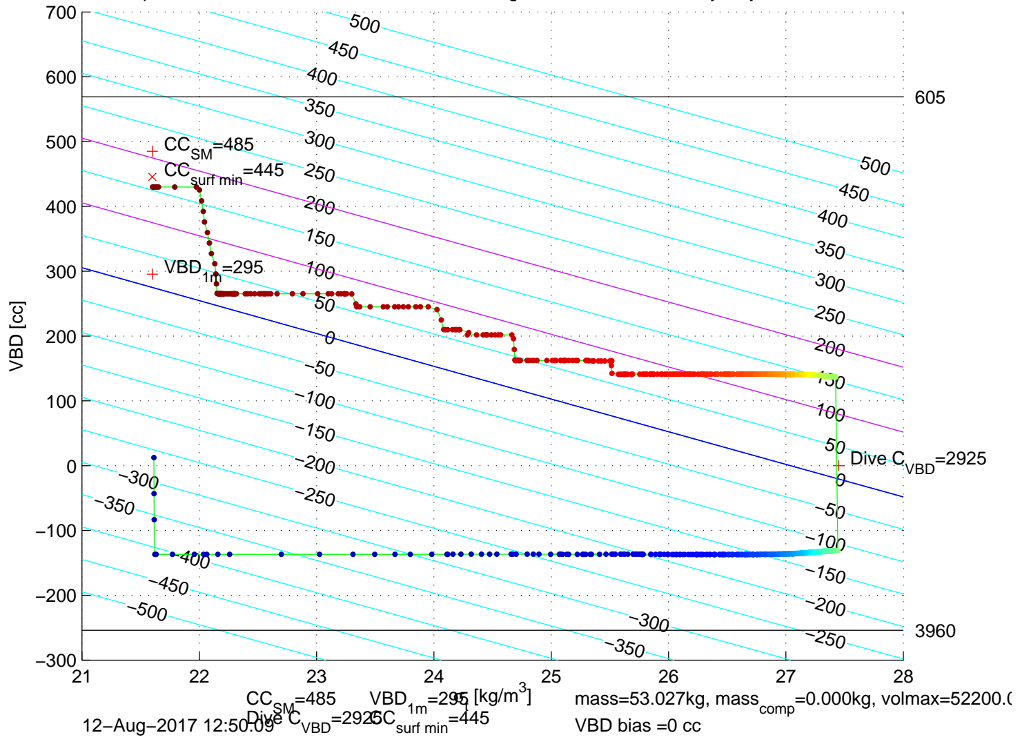
p6300216: SG630 Mission 7 Jul 2017 12-Aug-2017 12:51:46Z – buoyancy contoured
