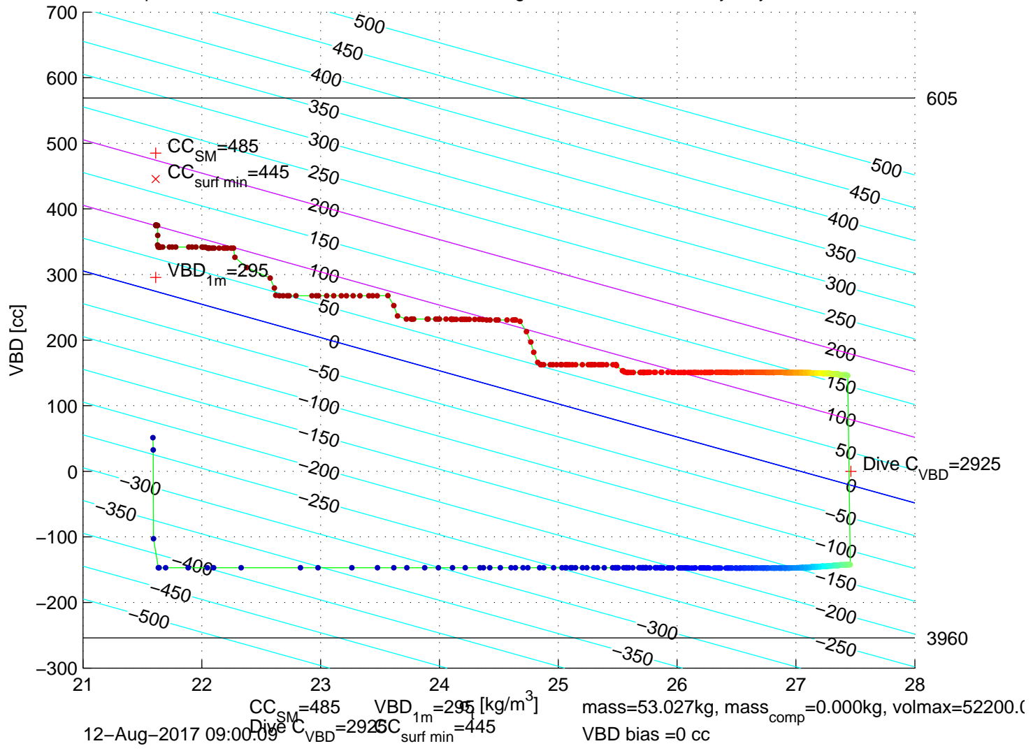
p6300215: SG630 Mission 7 Jul 2017 12-Aug-2017 09:11:29Z – buoyancy contoured
