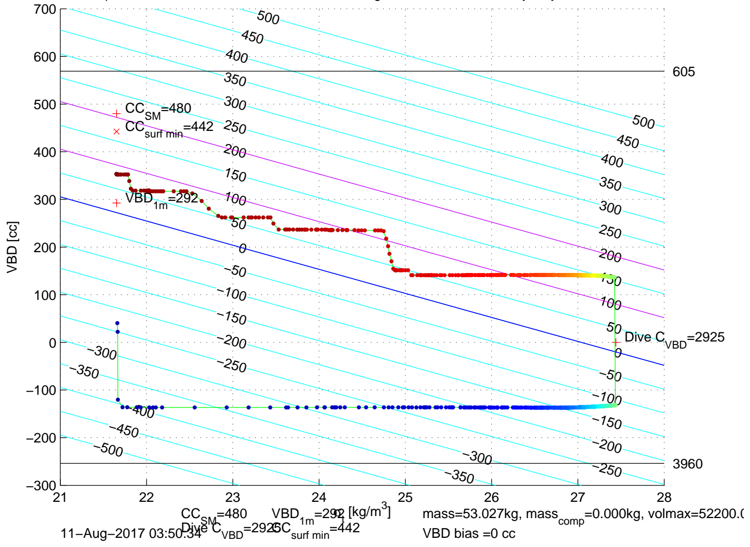
p6300207: SG630 Mission 7 Jul 2017 11-Aug-2017 03:53:30Z – buoyancy contoured
