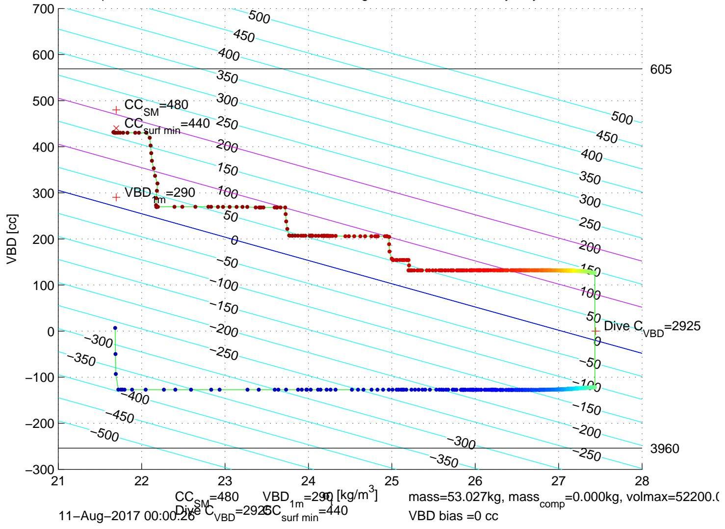
p6300206: SG630 Mission 7 Jul 2017 11-Aug-2017 00:05:15Z – buoyancy contoured
