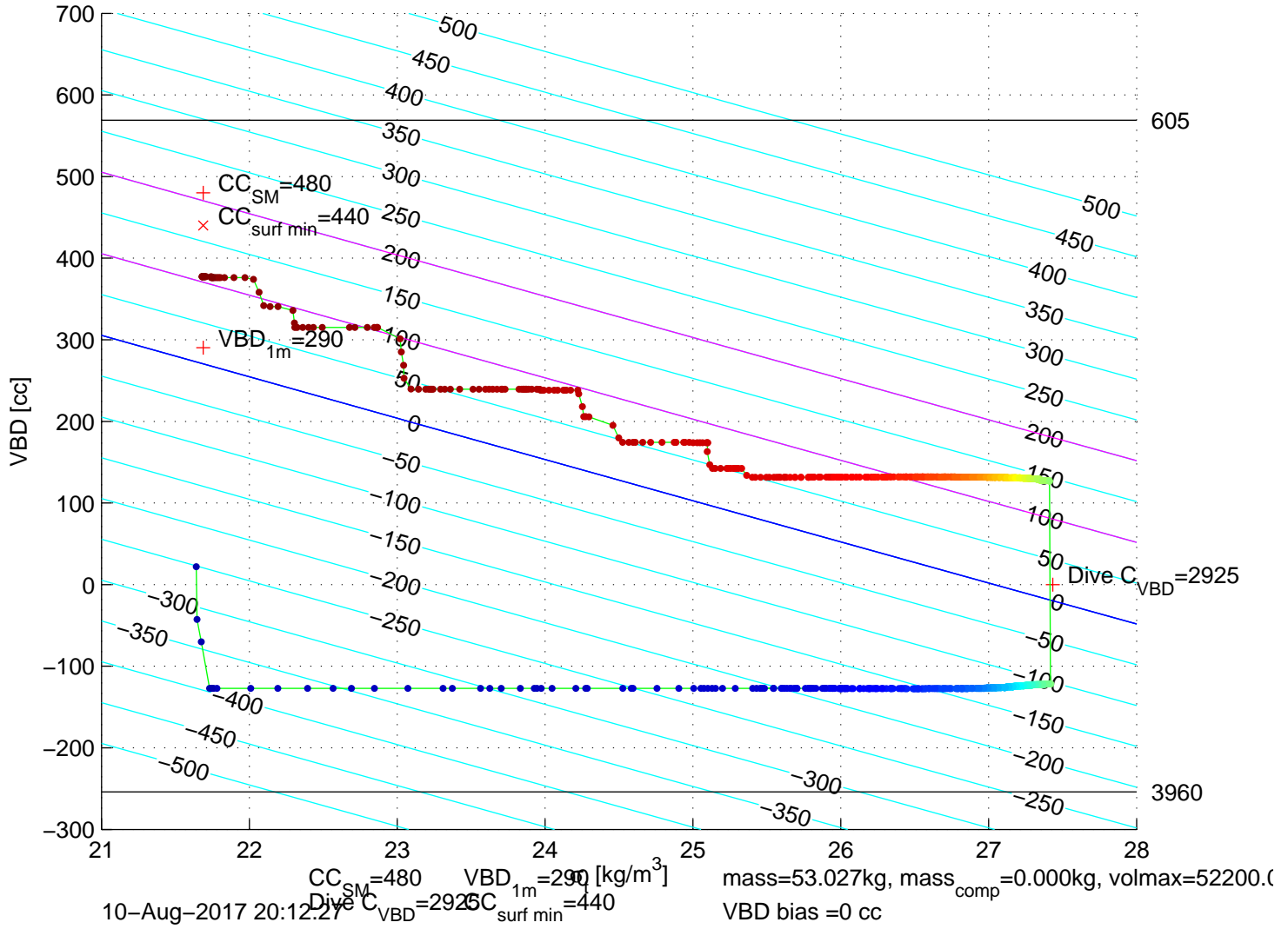
p6300205: SG630 Mission 7 Jul 2017 10–Aug–2017 20:11:56Z – buoyancy contoured
