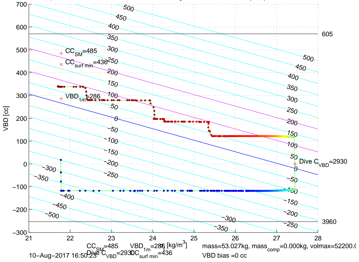
p6300203: SG630 Mission 7 Jul 2017 10–Aug–2017 12:21:29Z – buoyancy contoured
