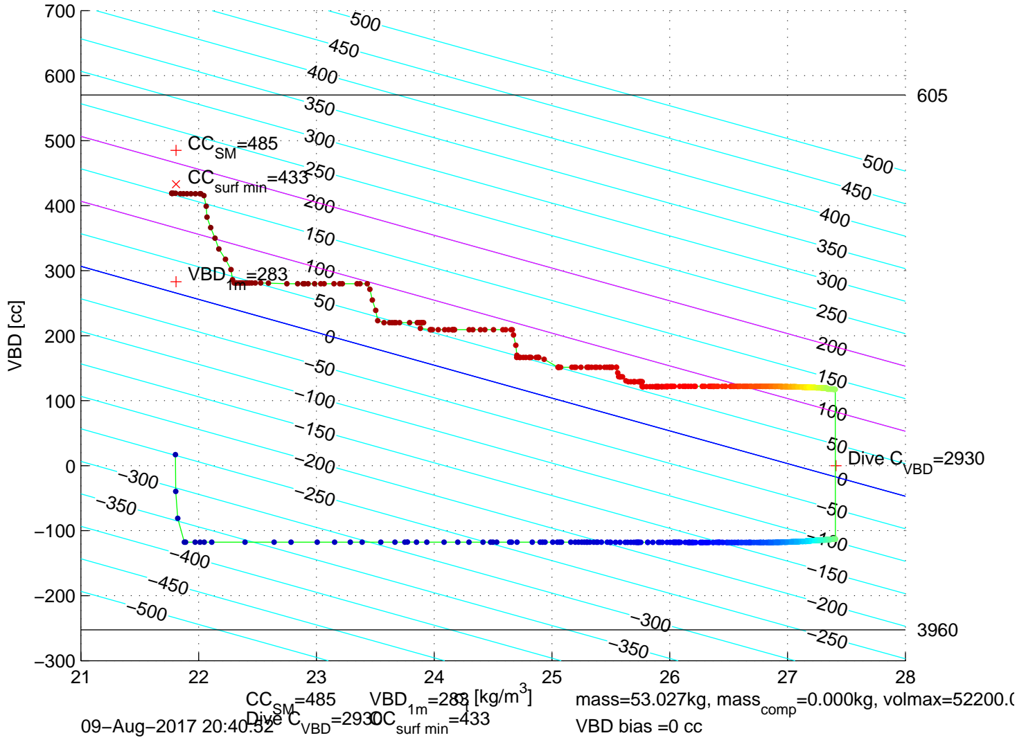
p6300199: SG630 Mission 7 Jul 2017 09–Aug–2017 20:37:10Z – buoyancy contoured
