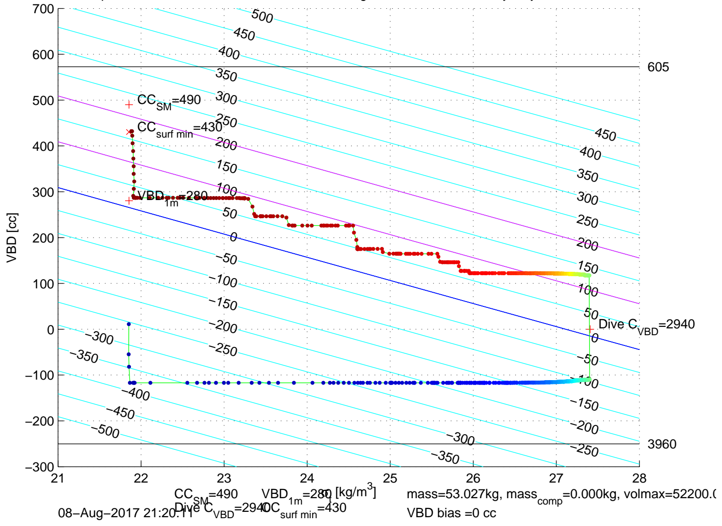
p6300193: SG630 Mission 7 Jul 2017 08-Aug-2017 21:16:21Z – buoyancy contoured
