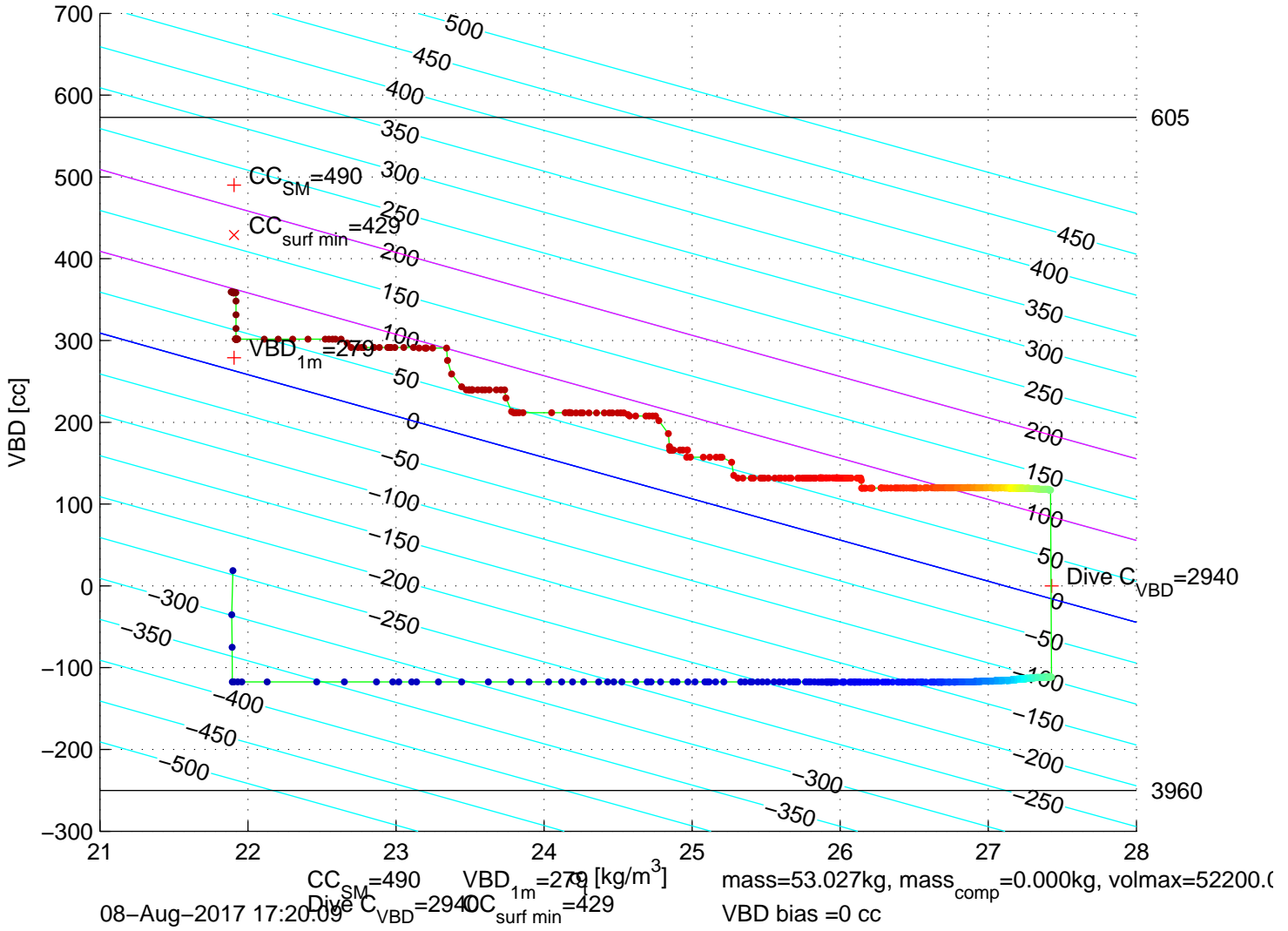
p6300191: SG630 Mission 7 Jul 2017 08-Aug-2017 12:59:20Z – buoyancy contoured
