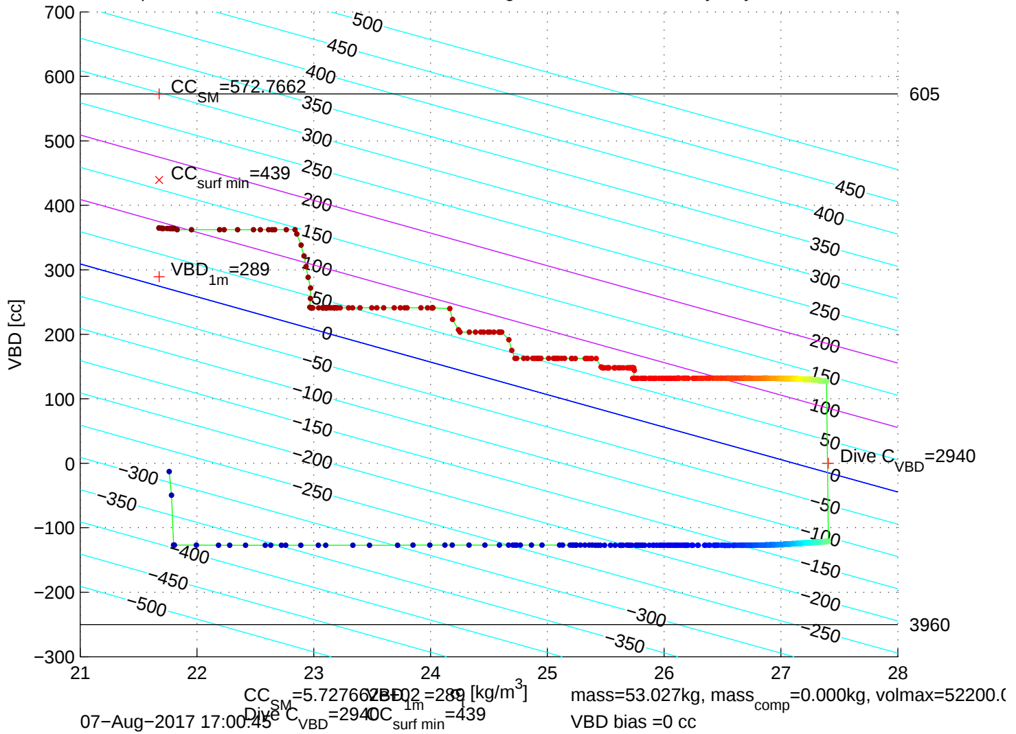
p6300186: SG630 Mission 7 Jul 2017 07-Aug-2017 16:51:25Z – buoyancy contoured
