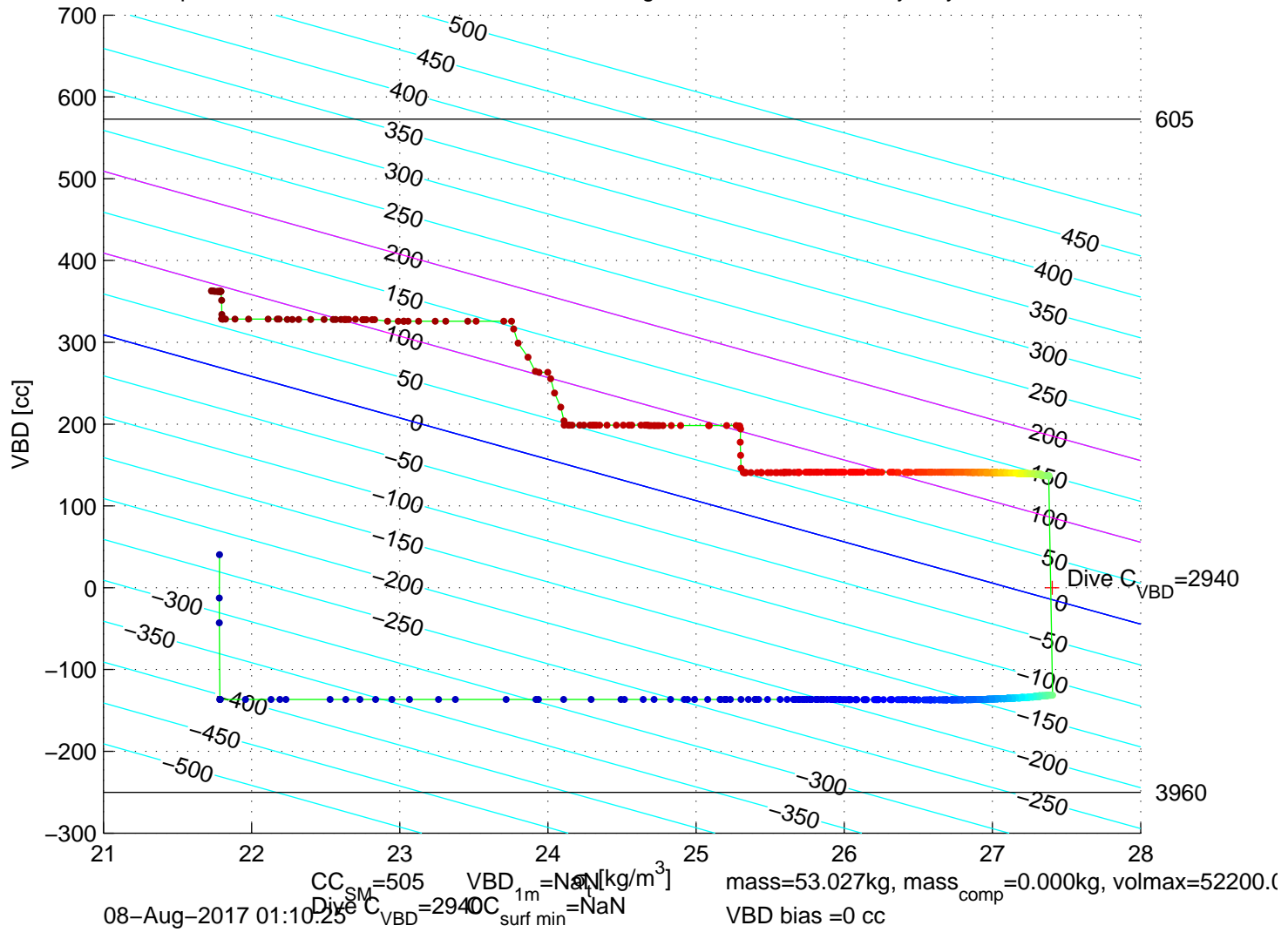
p6300185: SG630 Mission 7 Jul 2017 07-Aug-2017 13:04:11Z – buoyancy contoured
