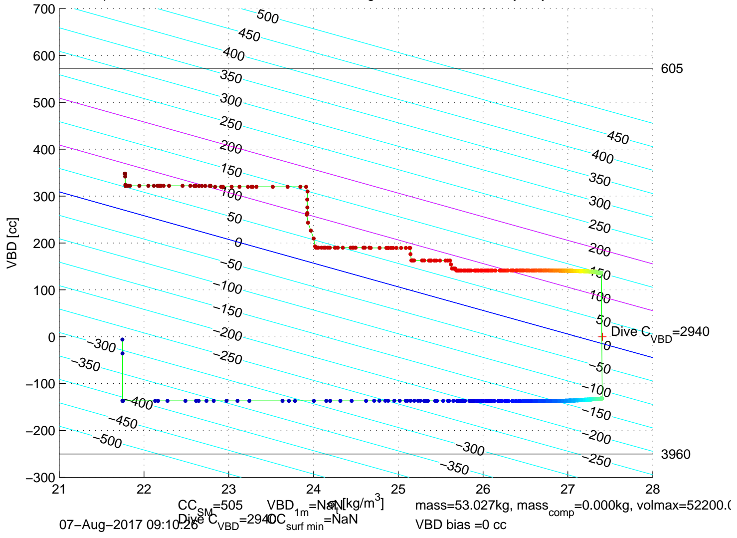
p6300184: SG630 Mission 7 Jul 2017 07-Aug-2017 09:23:30Z – buoyancy contoured
