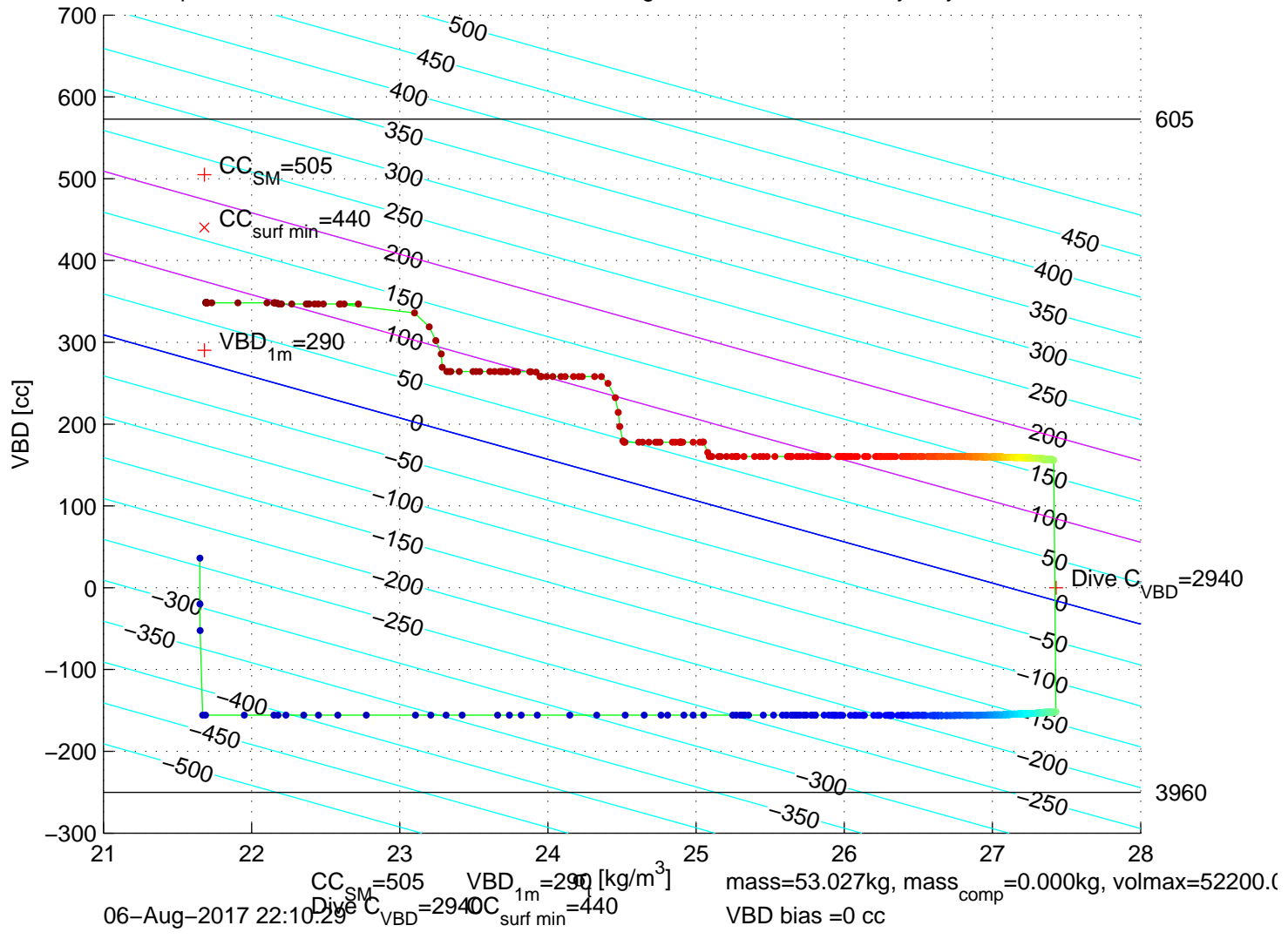
p6300181: SG630 Mission 7 Jul 2017 06–Aug–2017 22:36:49Z – buoyancy contoured
