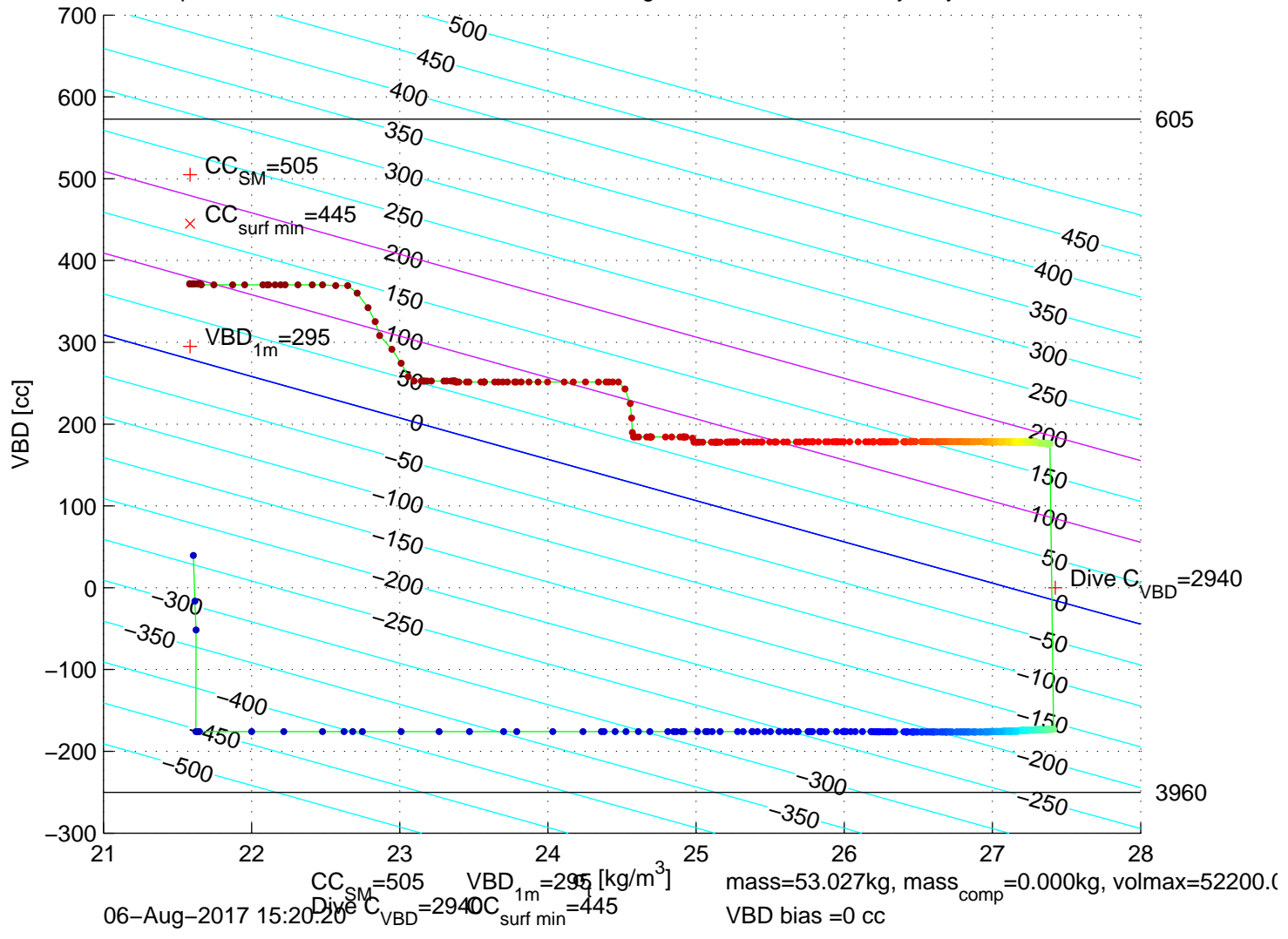
p6300179: SG630 Mission 7 Jul 2017 06–Aug–2017 16:02:07Z – buoyancy contoured
