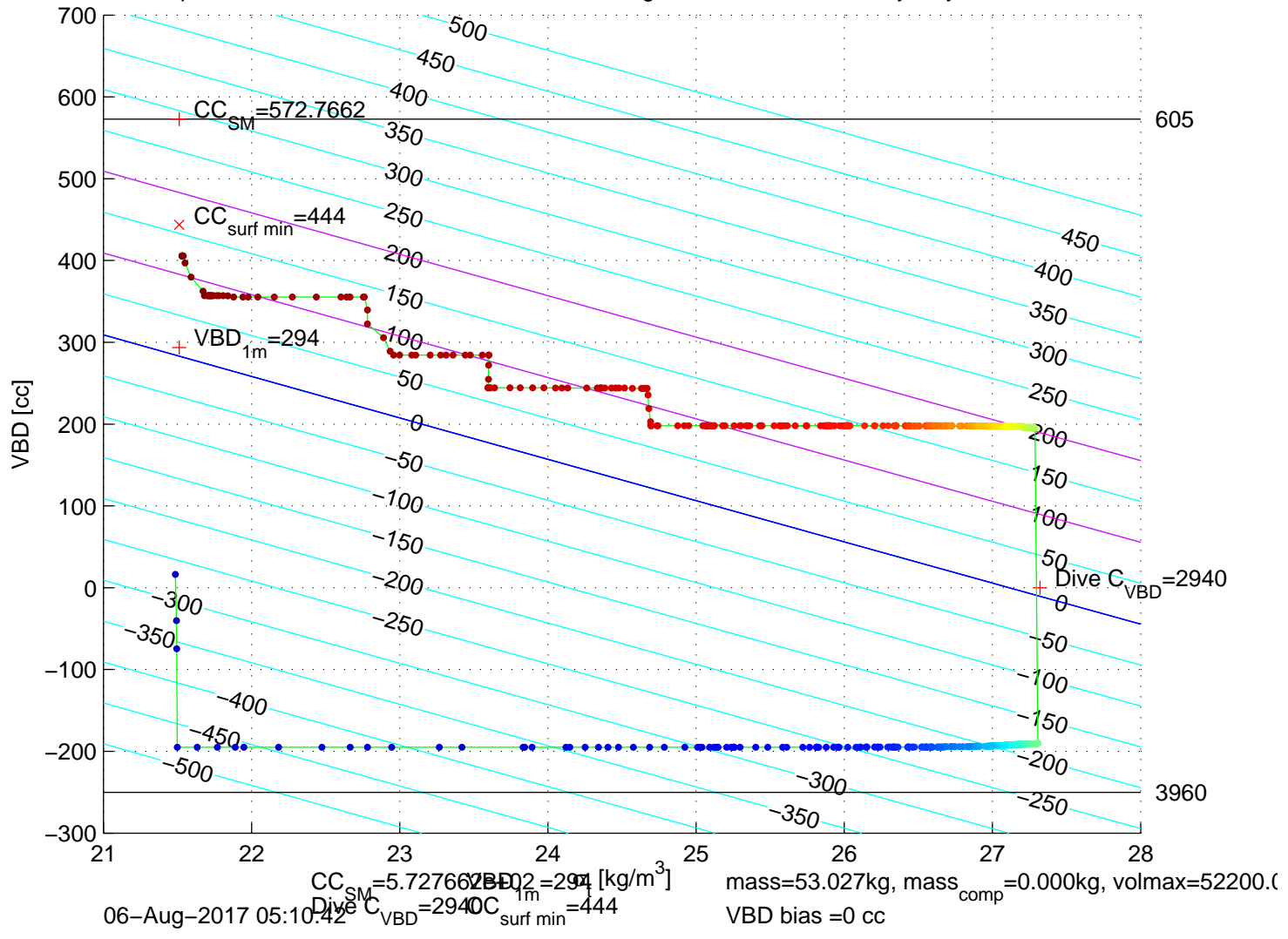
p6300176: SG630 Mission 7 Jul 2017 06-Aug-2017 06:07:54Z – buoyancy contoured
