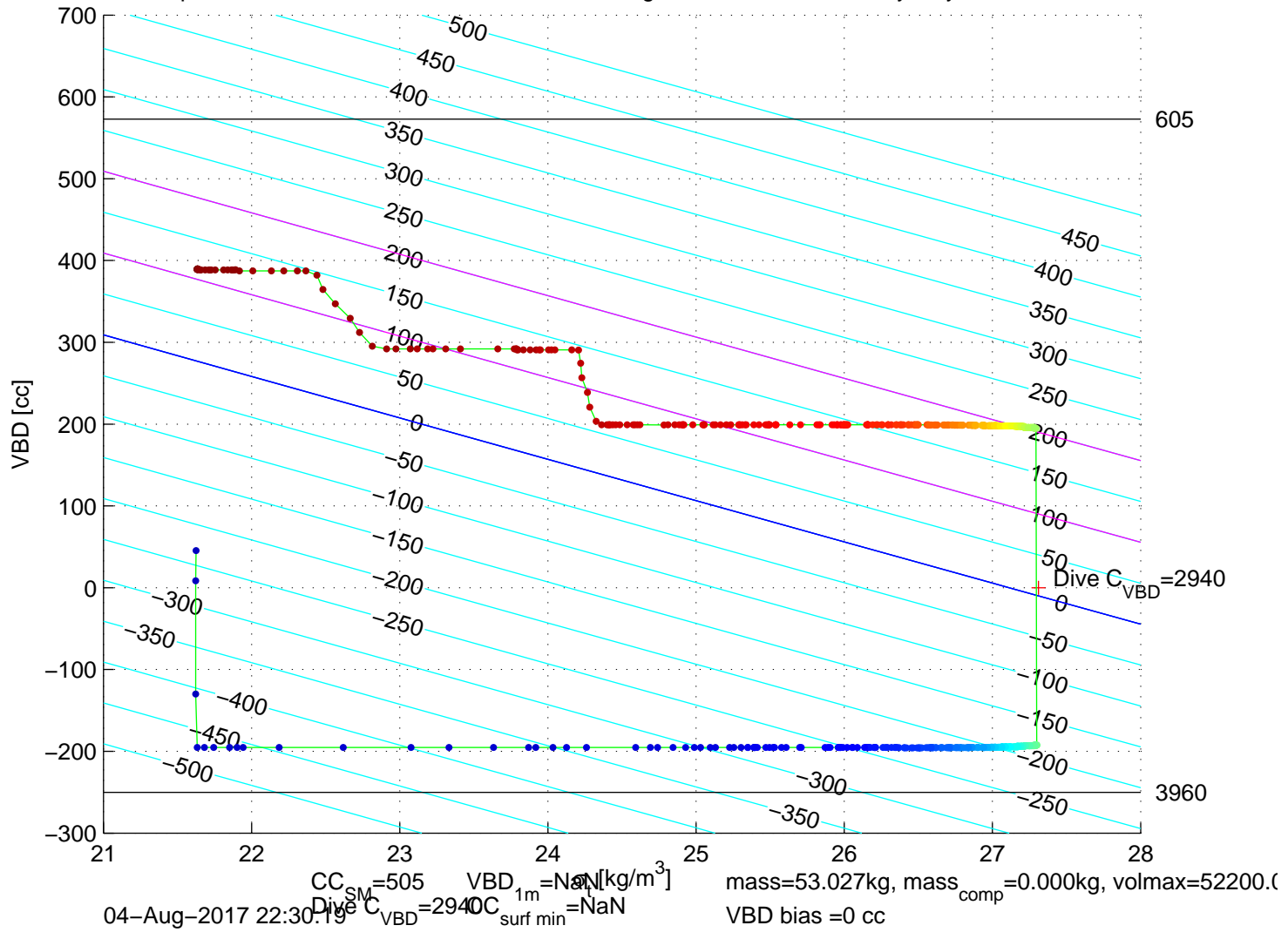
p6300165: SG630 Mission 7 Jul 2017 04-Aug-2017 23:46:01Z – buoyancy contoured
