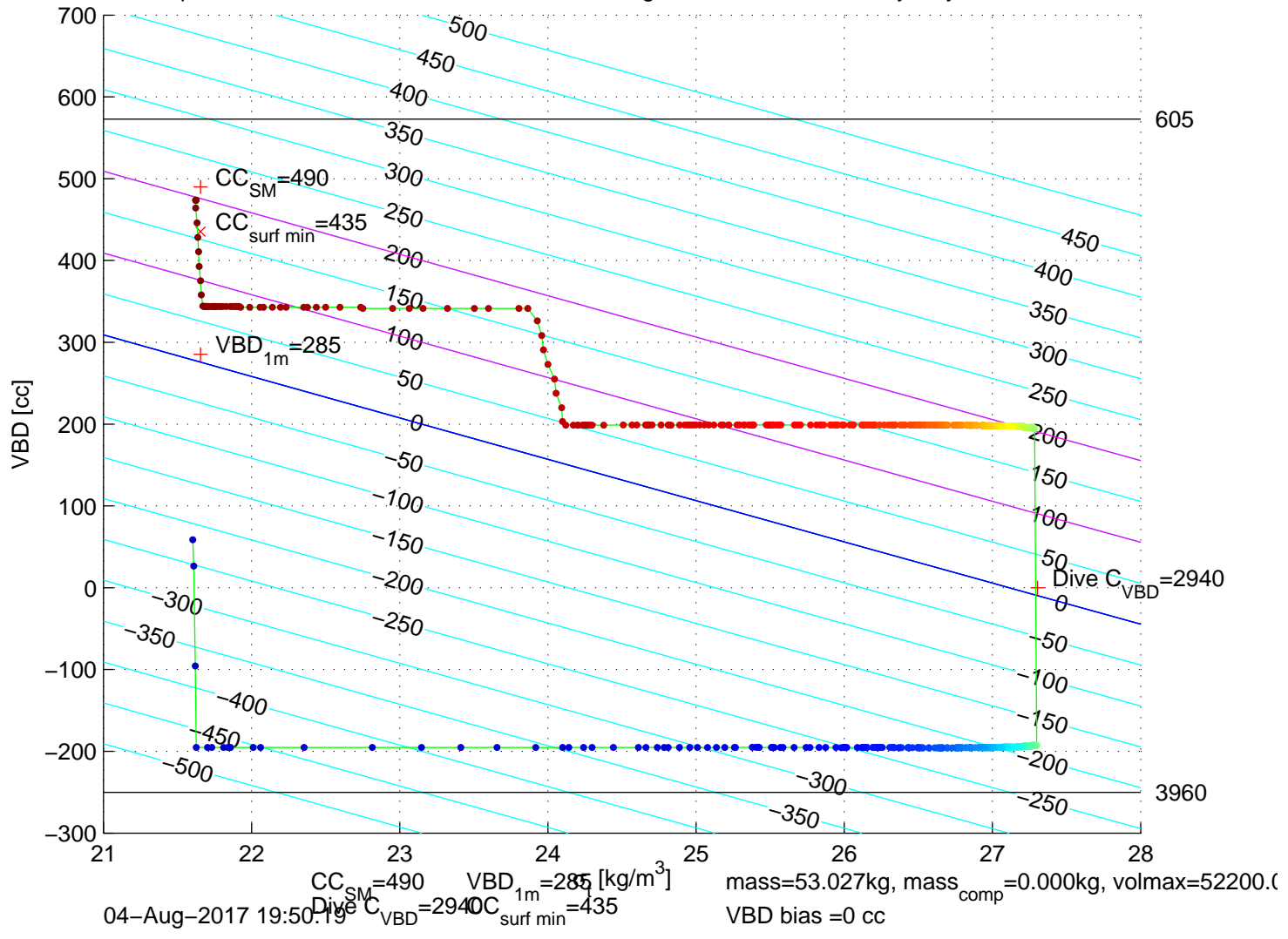
p6300164: SG630 Mission 7 Jul 2017 04–Aug–2017 20:59:03Z – buoyancy contoured
