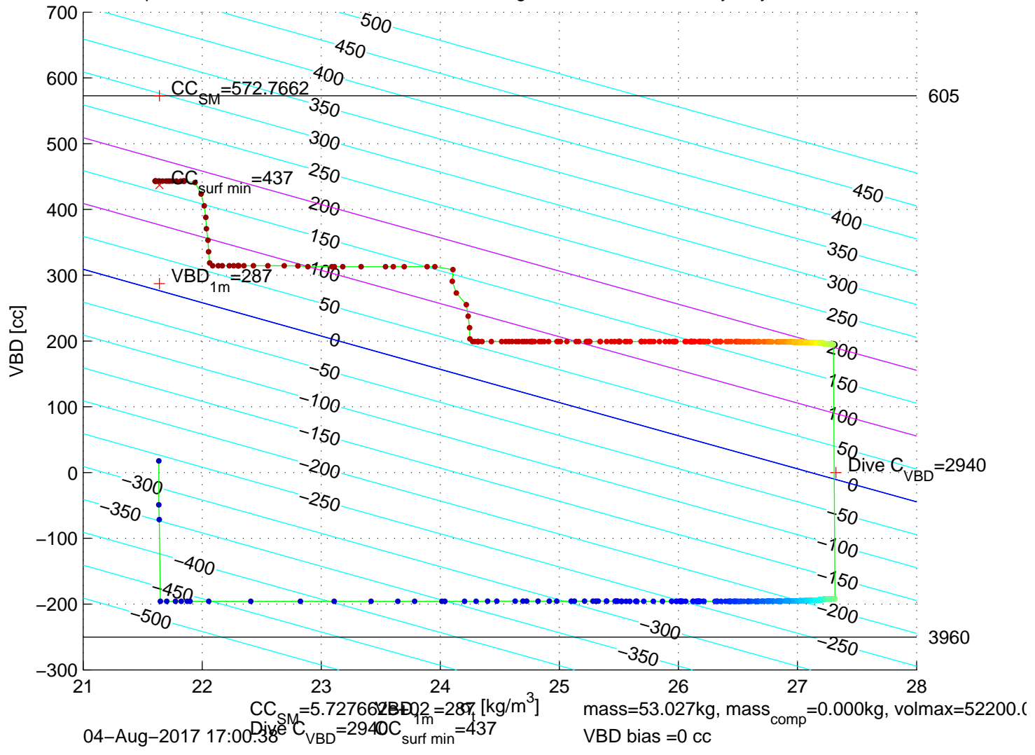
p6300163: SG630 Mission 7 Jul 2017 04-Aug-2017 18:18:22Z – buoyancy contoured
