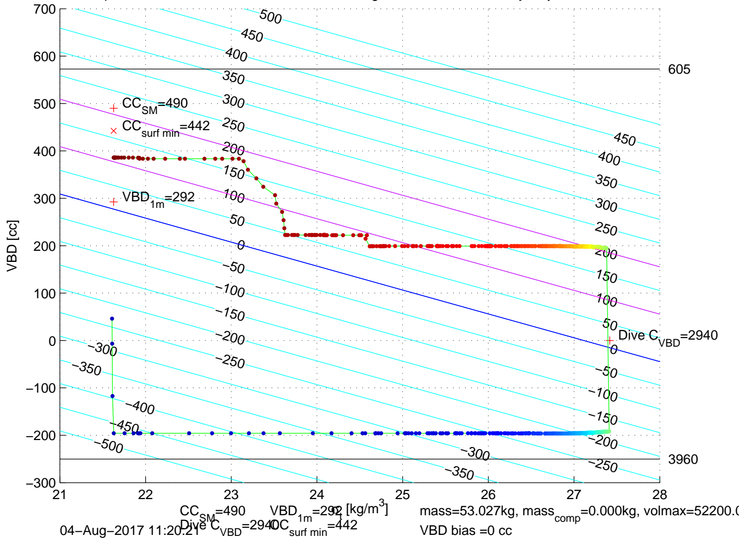
p6300161: SG630 Mission 7 Jul 2017 04-Aug-2017 12:11:05Z – buoyancy contoured
